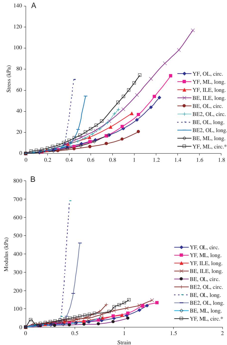
Fig. 12. Material properties of the bulbi of yellowfin and bigeye tuna. (A) Stress–strain curves. (B) Modulus–strain curves. The following rectangular tissue samples were stretched using a micromanipulator: YF, yellowfin tuna; BE, bigeye tuna; ML, segment of the middle layer; ILE, segment of longitudinal element; OL, segment of the outer layer; circ., stretched circumferentially; long., stretched longitudinally. The asterisk represents a tissue sample that was stretched as a loop using the custom-built stretching machine.
