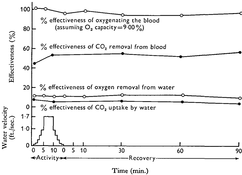
Fig. 1. The effectiveness of the exchange of oxygen and carbon dioxide between blood and water across the gills of rainbow trout during moderate exercise.
