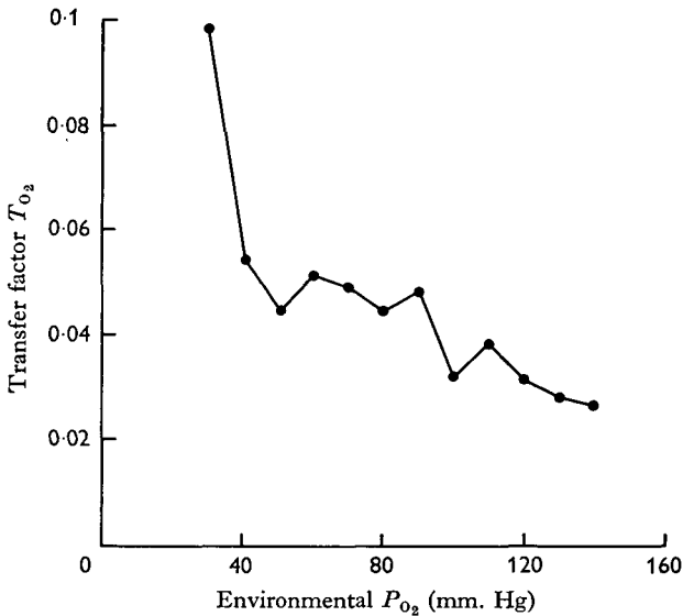
Fig. 5. Changes in the transfer factor of the gills for oxygen during hypoxia
