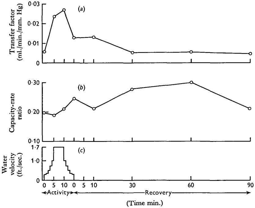
Fig. 3. Changes in the capacity-rate ratio and the transfer factor of the gills for oxygen during moderate exercise.
