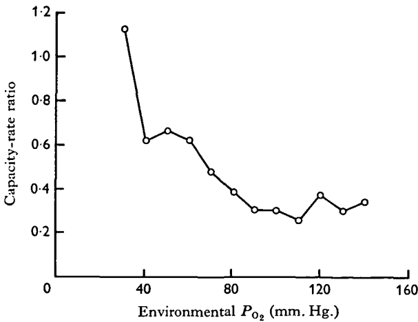
Fig. 4. Changes in capacity-rate ratio of blood to water at the gills during hypoxia
