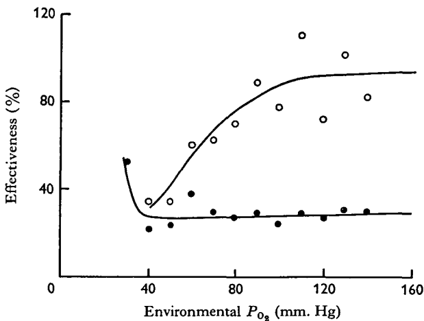
Fig. 2. The effectiveness of the exchange of oxygen between blood and water across the gills of rainbow trout during hypoxia. O, Oxygen loading by blood; ●, Oxygen removal from respiratory water.
