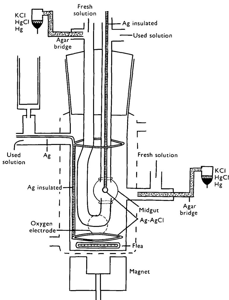
Fig. 1. Apparatus for short-circuiting the isolated midgut of Hyalophora cecropia . The potential is measured by calomel electrodes which connect via agar bridges to the solutions bathing blood-side and lumen of the isolated midgut. To short-circuit the midgut, an external potential is applied across the Ag-AgCl electrodes so that the small Ag-AgCl sphere in the centre of the midgut is negative. The placement of the midgut as a large sphere surrounding the central electrode ensures that the entire surface of the midgut is equipotential with respect to the lumen solution. The potential gradient in the blood-side solution is kept as uniform as possible by forming the Ag-AgCl electrode as two large rings placed symmetrically as far as possible from the gut. The midgut is made a sphere by adjusting the volume of fluid in the outer compartment by means of the syringe. The dotted circle shows the location of the oxygen electrode near the stirrer in the wall of the outer compartment. A short section of iron rod enclosed in glass tubing serves as a stirrer. The entire outer compartment is enclosed in a glass jacket (dotted line) through which water is circulated from a constant temperature circulator.
