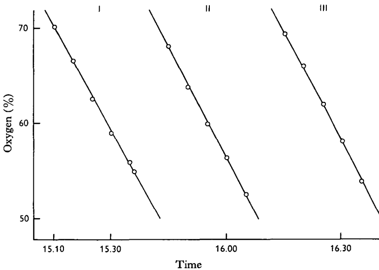
Fig. 2. A representative experiment in which the time-course of oxygen uptake is plotted when the midgut is transporting potassium (period II) and when the potassium transport has been stopped (periods I and III). In period II, the midgut is producing a short-circuit current of 1400 \mu A. (equivalent to 47 \mu -equiv. potassium/h. if 90% of the current is carried by potassium). In periods I and III an external potential of 60 mV. is added to the natural potential, making the lumen about 150 mV. positive to the blood side. The rate of oxygen uptake as indicated by the slope of the lines is virtually identical under the two conditions.
