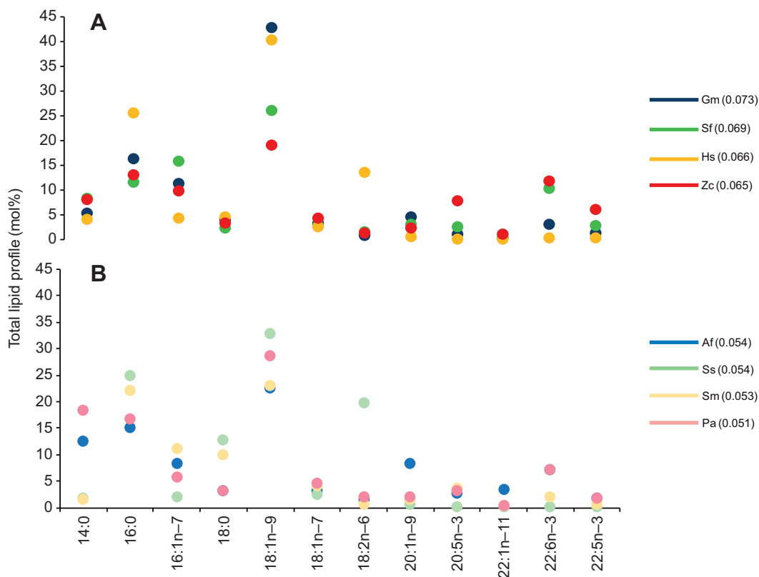
Fig. 4. The 12 most abundant FA (mol%) in the lipid profiles and N_2 solubility ( ml N_2 ml^{-1} oil). (A) The samples with the four highest N_2 solubility values (Gm, short-finned pilot whale; Sf, Atlantic spotted dolphin; Hs, human; Zc, California sea lion). (B) The samples with the four lowest N_2 solubility values (Af, emperor penguin; Ss, pig; Sm, eider duck; Pa, Adélie penguin). Data for the short-finned pilot whale and the Atlantic spotted dolphin are from Lonati et al. (2015) and data for the human and pig are from Gabler-Smith et al. (2020).
