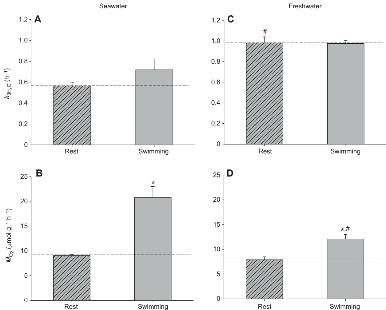
Fig. 3. The effects of steady-state exercise on rates of diffusive water exchange ( k_{3H_2O} , Series 2) and oxygen consumption ( \dot{M}_{O_2} ) of killifish acclimated to either seawater or freshwater. (A) Diffusive water exchange in seawater. (B) Oxygen consumption in seawater. (C) Diffusive water exchange in freshwater. (D) Oxygen consumption in freshwater. Measurements were made at rest or during 1 h of swimming at 2 body lengths s^{-1} . Data are means \pm 1 s.e.m. ( N=8 different fish in each treatment, for each measured parameter). Other details as in legend of Fig. 1. For k_{3H_2O} , there were overall significant effects of salinity but not swimming, whereas for \dot{M}_{O_2} there were overall significant effects of swimming but not salinity, as well as significant interaction.
