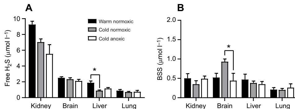
Fig. 1. Free \text{H}_2\text{S} and bound sulfane sulfur (BSS) in tissues of Trachemys scripta elegans . Tissue concentration of (A) free \text{H}_2\text{S} and (B) BSS in warm normoxic turtles ( N=5 brain, liver, lung; N=3 kidney) and cold normoxic turtles ( N=5 brain, liver, lung; N=4 kidney) and cold anoxic turtles ( N=4 for all tissues). Data are means \pm s.e.m. Significant differences (ANOVA/Kruskal–Wallis tests) are indicated (* P<0.05 ).
