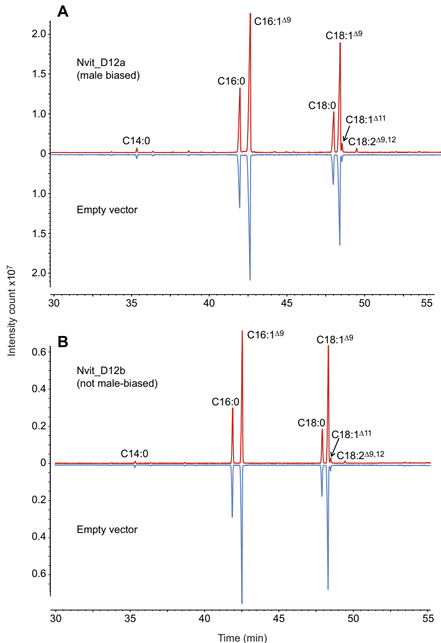
Fig. 2. Transformed yeast cells expressing Nvit_D12a or Nvit_12b synthesise C18:2 Δ9,12 . GC/MS analysis on a polar BP-20 column of FAMEs extracted from transformed S. cerevisiae cells supplemented with C18:1 Δ9 . Cells were transformed with (A) Nvit_D12a and (B) Nvit_D12b. Cells carrying the empty vector were used as controls. The results are representative of three replicate experiments.
