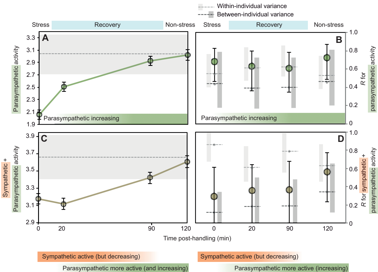
Fig. 2. Changes in autonomic indexes (from heart rate variability) between periods of stress and non-stress in streaked shearwaters and consistent individual differences. (A) Mean ( \pm 95\% CI) parasympathetic ‘rest-and-digest’ activity post-handling (log rMSSD index of heart rate variability on y-axis), during a 2 h recovery period in nests ( n=195 ). The grey dashed line reflects baseline mean (shading: \pm 95\% CI). (B) Individual within-year repeatability (circles) \pm 95\% CIs and within-/between-individual standardized variance components \pm 95\% CIs for parasympathetic activity (log rMSSD) post-handling ( n=120-123 ). (C) Mean ( \pm 95\% CI) combined sympathetic ‘fight-or-flight’+parasympathetic rest-and-digest activity (represented by log SDNN index of heart rate variability) post-handling, during a 2 h recovery period in nests ( n=195 ). The grey dashed line reflects baseline mean (shading: \pm 95\% CI). (D) Individual within-year repeatability (circles) \pm 95\% CIs and within-/between-individual standardized variance components \pm 95\% CIs for combined sympathetic fight-or-flight+parasympathetic rest-and-digest activity (log SDNN) post-handling ( n=123, 122, 123, 120 for 0, 20, 90 and 120 min, respectively).
