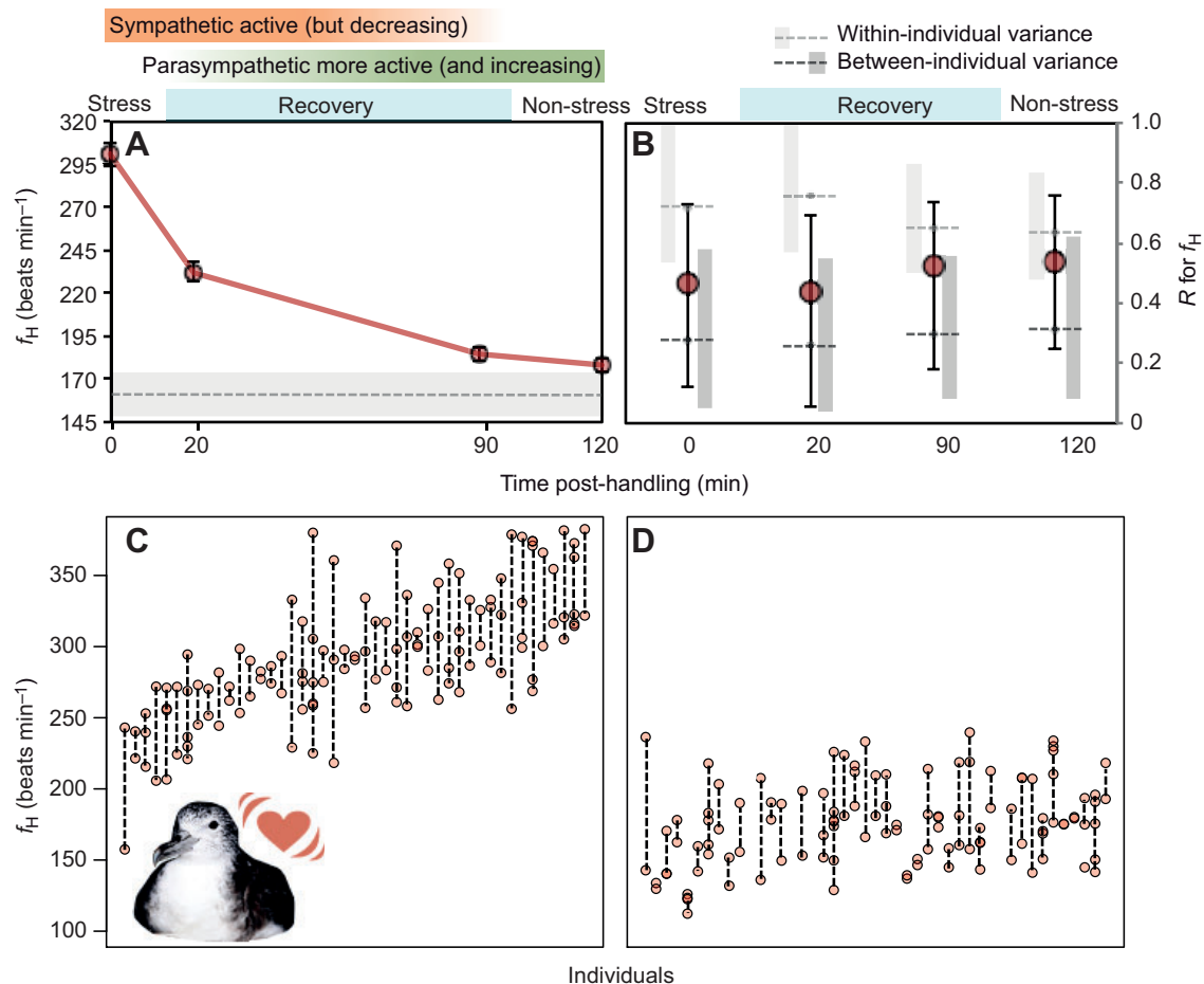
Fig. 1. Changes in heart rate between periods of stress and non-stress in streaked shearwaters and consistent individual differences. (A) Mean ( \pm 95\% confidence interval, CI) heart rate ( f_H ) post-handling, during a 2 h recovery period in nests ( n=195 ). The grey dashed line reflects baseline mean (shading: \pm 95\% CI) from a previous study where loggers were kept on incubating birds for 24 h (Müller et al., 2017). (B) Repeatability ( R ) is a standardized index ranging between 0 and 1 that reflects consistent individual differences and is calculated as between-individual variation divided by the sum of between-individual and within-individual variation, in a phenotypic trait. Individual within-year repeatability (circles) \pm 95\% CIs and within-/between-individual standardized variance components \pm 95\% CIs for heart rate post-handling ( n=123, 122, 123, 120 for 0, 20, 90 and 120 min, respectively) are shown. (C,D) Individual differences in heart rate. Vertically connected points are heart rate values from repeated tests of 45 individuals (same year), 0 min (stress; C) and 120 min (non-stress, baseline; D) post-handling.
