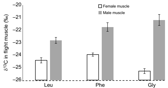
Fig. 3. \delta^{13}\text{C} in the flight muscle of male and female moths fed one of three ^{13}\text{C} -labeled AAs in nectar. n=5 males and n=5 females for each AA. Error bars are 1 s.e.m. The dashed horizontal line signifies the background \delta^{13}\text{C} value of control moths fed the standard diet without ^{13}\text{C} -tracers. A less-negative number indicates more tracer. Kruskal–Wallis rank sums test between sexes: Gly, P=0.0122 ; Leu, P=0.0122 ; Phe, P=0.0358 .
