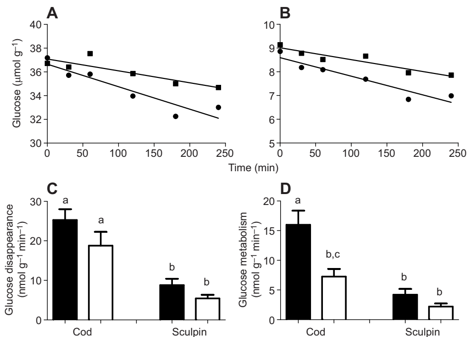
Fig. 6. Glucose disappearance from medium and glucose metabolism. Atlantic cod myocytes were incubated with 5 \text{ mmol l}^{-1} glucose and short-horned sculpin with 0.5 \text{ mmol l}^{-1} glucose in medium. Experiments were conducted at 8^\circ\text{C} . (A,B) Examples of the relationship between glucose disappearance and time for Atlantic cod (A) and short-horned sculpin (B). Circles, control; squares, cytochalasin B. (C) Glucose disappearance ( N=7 for both species). (D) Glucose metabolism, measured by ^3\text{H}_2\text{O} production from [2\text{-}^3\text{H}]\text{glucose} ( N=7 for Atlantic cod; N=5 for short-horned sculpin). For C and D, filled bars, control; open bars, cytochalasin B. Statistical significance was assessed as described for Fig. 5. Values sharing a letter are not significantly different.
