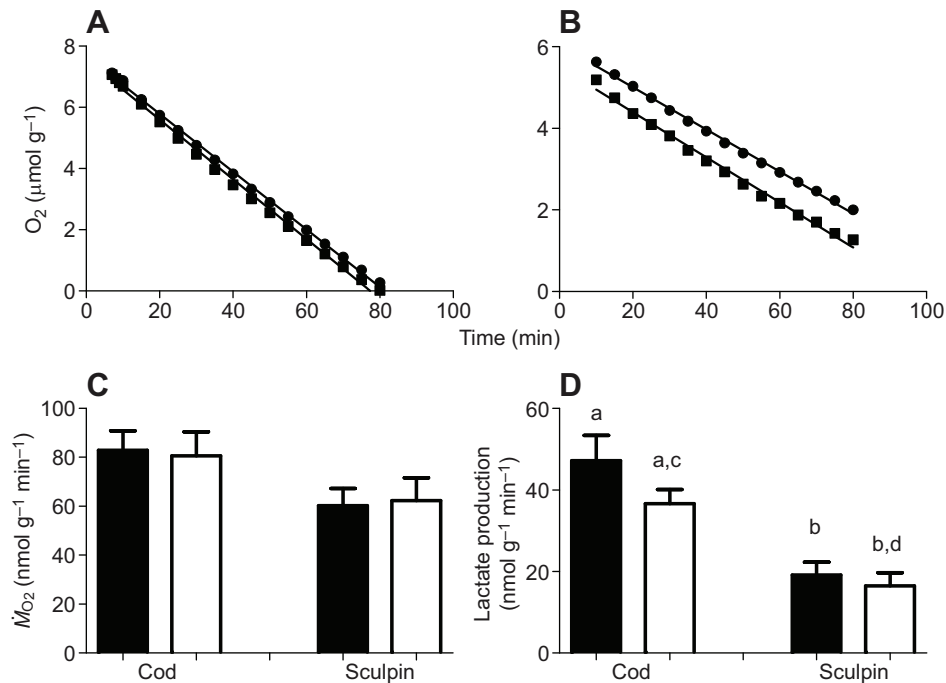
Fig. 5. Oxygen consumption and lactate production by isolated myocytes. Atlantic cod myocytes were incubated in 5 \text{ mmol l}^{-1} glucose and short-horned sculpin in 0.5 \text{ mmol l}^{-1} glucose in medium. Experiments were conducted at 8^\circ\text{C} . (A,B) Examples of the relationship between oxygen content and time for Atlantic cod (A) and short-horned sculpin (B) myocytes incubated in closed chambers. Oxygen level in the medium was normalized to grams wet mass of cells. Circles, control; squares, cytochalasin B. (C) Oxygen consumption ( \dot{M}_{\text{O}_2} ; N=6 for both species). (D) Lactate production ( N=7 for both species). For C and D, filled bars, control; open bars, cytochalasin B. Statistically significant differences between species were assessed with a two-way ANOVA and the impact of cytochalasin B treatment with repeated measures two-way ANOVA with the Bonferroni post-test applied in both cases. Values sharing a letter are not significantly different.
