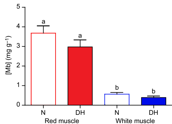
Fig. 4. Myoglobin (Mb) concentration in red and white muscle from normoxic and deeply hypoxic crucian carp. Mb concentration is given in mg per g wet mass for crucian carp exposed to normoxia (N; P_{O_2} > 140 mmHg) and deep hypoxia (DH; 1 < P_{O_2} < 3 mmHg) for 1 day. Values are means \pm s.e.m. ( N=15 for each group). Differences between groups were tested using a one-way ANOVA, followed by a Bonferroni post hoc test, and different letters signify statistical differences between groups.
