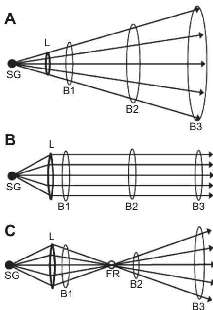
Fig. 1. Different patterns of beam attenuation with distance. (A) Unfocused beam from a point source and ideal spherical spreading. Absolute beamwidth increases with distance, but angular beamwidth remains constant. (B) Ideally focused beam in which absolute beamwidth remains constant irrespective of distance, but angular beamwidth decreases with distance. (C) Convergent beam resulting in a focal region (FR) and variable angular beamwidth measurements. SG, sound generator; L, focusing lens; B1–B3, variable beamwidths at different distances from the sound source.
