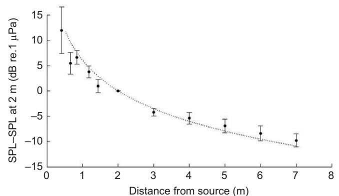
Fig. 2. Recording signals along the beam axis. See Fig. 7B for the experimental configuration. Relative sound pressure level (SPL, in dB re. 1 μPa) measured at a distance from the sound source for 614 clicks from 30 click trains. The circles represent the mean difference between the SPL measured at a given distance ( r ) and the SPL measured at 2 m, and the bars represent the s.d. of each point. The dashed curve represents the spherical spreading loss function of 1/r , with a reference at 2 m.
