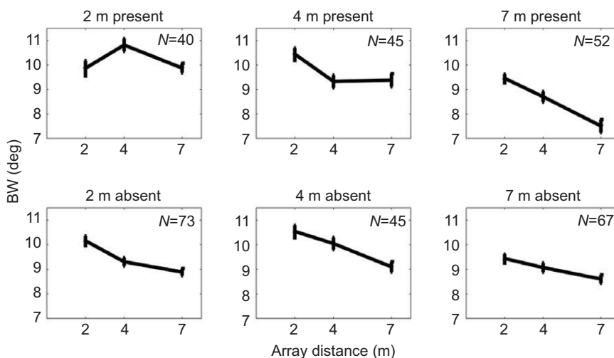
Fig. 3. Mean \pm s.e. -3 dB beamwidth after cubic interpolation across the three recording arrays for each target condition. BW, beamwidth.
