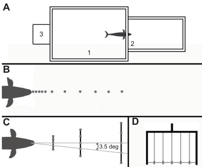
Fig. 7. Experimental setup and array configurations. (A) Topside view of the experimental pen (1), target pen (2) and trainer/equipment shack (3). (B) Topside view for near-to-far field transition determination with the hydrophones located at 1 m depth and at distances of 0.5, 0.75, 1, 1.25, 1.5, 2, 3, 4, 5, 6 and 7 m from the blowhole. Hydrophone elements are indicated by the gray circles. (C) Topside view of linear arrays with the arrays located at 1 m depth and 2, 4 and 7 m distance. Hydrophone elements are indicated by the gray circles, and the PVC framework is indicated by the black lines. The inter-sensor spacing was chosen to maintain angular spacing of approximately 3.5 deg for each array. (D) Forward view of one array from the whale's perspective. Hydrophone elements are indicated by the gray oblongs, the PVC framework is indicated by the black lines, and the monofilament is indicated by the dotted lines.
