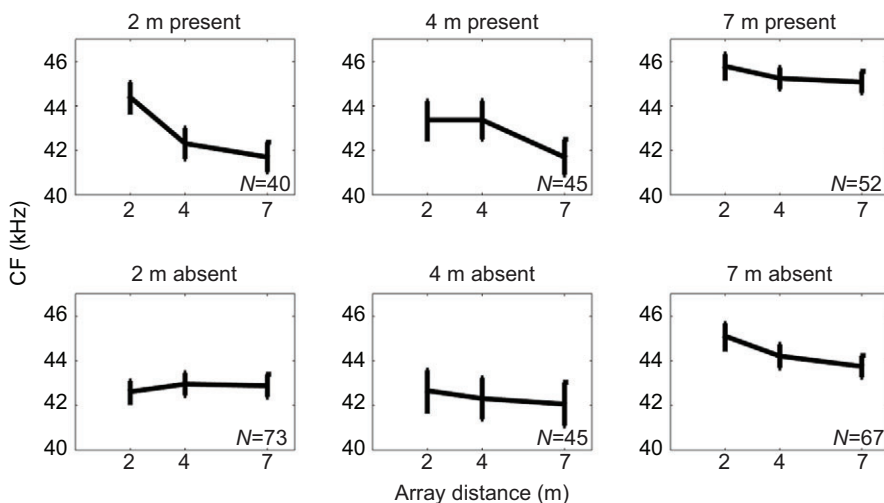
Fig. 5. Mean \pm s.e. center frequency after cubic interpolation across the three recording arrays for each target condition. CF, center frequency.
