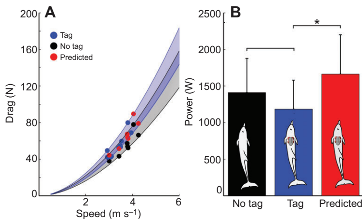
Fig. 1. Bio-logging tags increase the drag forces experienced by bottlenose dolphins. (A) Envelope of the drag force (N) estimated for the four bottlenose dolphins in this study when not wearing (black) and wearing (blue) bio-logging tags across a range of swimming speeds (lines; \text{m s}^{-1} ) and for specific observed swimming speeds (dots; \text{m s}^{-1} ). Red dots reflect the predicted drag loading in the tagged condition if individuals maintained their non-tagged swimming speed. (B) Mean \pm s.d. power output (W) estimated for when (blue) wearing a tag, swimming at observed speeds; and (black) not wearing a tag, swimming at observed speeds; and predicted for when (red) wearing a tag, if individuals had maintained their non-tagged swimming speed.
