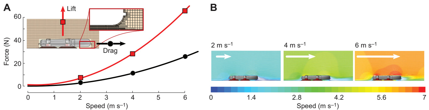
Fig. 4. Lift and drag forces on a DTAG2 increase with speed. (A) Lift (red) and drag (black) forces (N) on a DTAG2, and (B) flow visualization at uniform velocity profiles of 2, 4 and 6 m s -1 from computational fluid dynamics (CFD) simulations using STAR-CCM+ (version 9.04) over 9.6 m cells, with extra mesh refinement in the region located under the tag (A). See main text for further CFD details.
