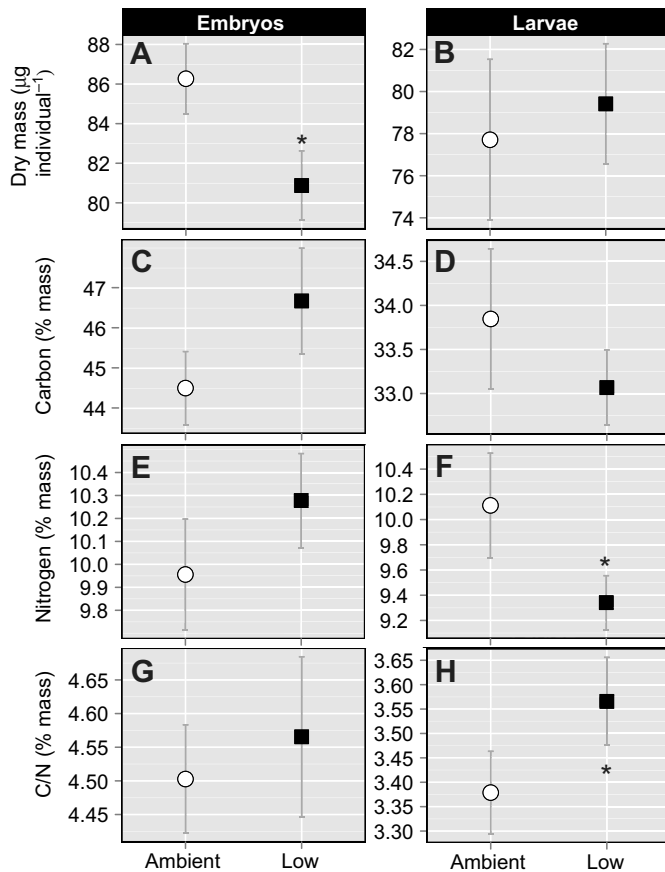
Fig. 4. (A,B) Dry mass, (C,D) carbon, (E,F) nitrogen and (G,H) carbon/nitrogen (C/N) ratio of P. cinctipes embryos and larvae reared in ambient pH ( 7.93 \pm 0.06 ) or low pH ( 7.58 \pm 0.06 ). Each point represents the mean \pm s.e.m. for N=33-35 individuals for embryos (after 5–7 days exposure) and N=15-19 individuals for larvae (after 6 days exposure). *Significant difference ( P \leq 0.05 ) between pH treatments within a developmental stage.
