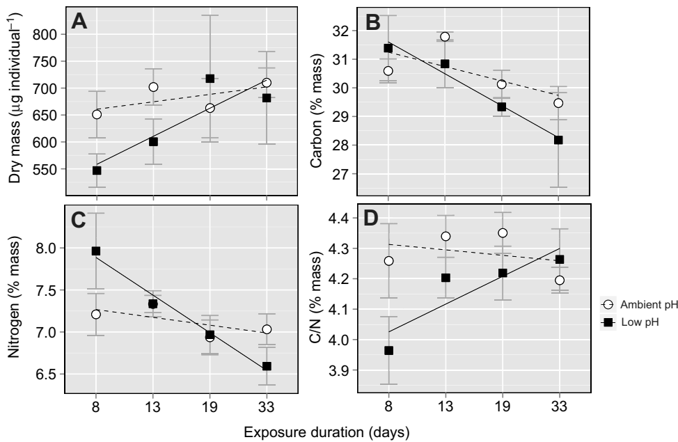
Fig. 5. Juvenile P. cinctipes (A) dry mass, (B) carbon content, (C) nitrogen content and (D) C/N of individuals reared in ambient pH ( 7.93 \pm 0.06 ) or low pH ( 7.58 \pm 0.06 ) (different individuals sampled for each time point). Each point represents the mean \pm s.e.m. for N=4-6 individuals. Statistical analysis indicated a minor effect of pH on C/N (ANOVA, F_{1,36}=4.0 , P=0.05 ).
