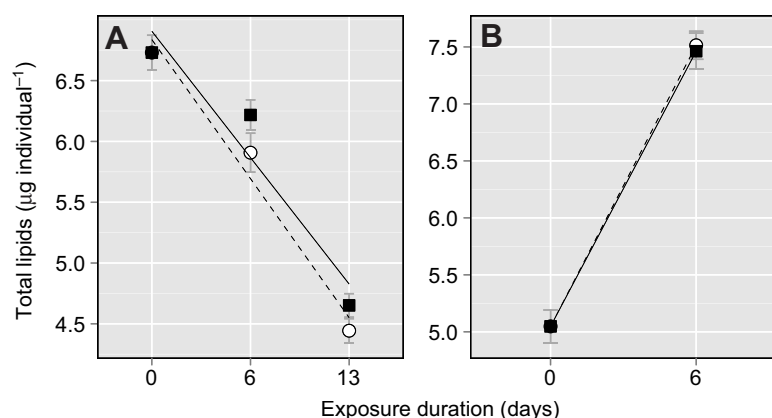
Fig. 6. Petrolisthes cinctipes total lipids in (A) embryos after 0, 6 and 13 days and (B) larvae after 0 and 6 days in individuals reared in ambient pH (7.93±0.06) or low pH (7.58±0.06). Each point represents the mean ± s.e.m. for N=30-32 individuals for embryos and N=15-16 individuals for larvae. Analysis indicated no significant differences between treatments for embryos (ANOVA, F_{1,181}=3.8 , P=0.07 ) and larvae (ANOVA, F_{1,60}=0.03 , P=0.85 ).
