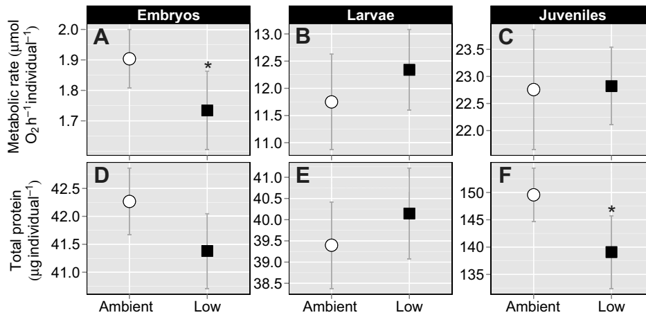
Fig. 1. (A–C) Oxygen consumption rate and (D–F) total protein at embryo, zoea I larvae and early juvenile stages of Petrolisthes cinctipes after short-term exposure (embryos 7–10 days, larvae 4–10 days, juveniles 3–5 days) to ambient pH ( 7.93 \pm 0.06 ) or low pH ( 7.58 \pm 0.06 ). Each point represents the mean \pm s.e.m. for N=54 – 55 individuals for embryos, N=50 individuals for larvae and N=23 – 24 individuals for juveniles. Individuals were pooled from six broods for embryos and larvae (females used for hatching out larvae were different from those from which we obtained embryos). *Significant difference ( P \leq 0.05 ) between pH treatments within a developmental stage. For embryos and larvae, statistical analyses were performed on data normalized to the mean oxygen consumption rate per brood to remove variation due to differences in basal metabolism among clutches.
