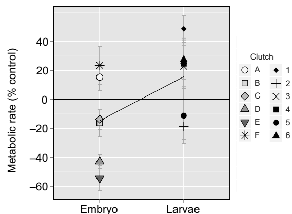
Fig. 3. Effect of changes in pH ( \Delta\text{pH} ) on the metabolism of P. cinctipes embryos and zoea I larvae, presented as the percentage difference in oxygen consumption rate per individual between low pH (7.58±0.06)-reared individuals and ambient pH (7.93±0.06)-reared individuals for each brood. Effect of \Delta\text{pH} becomes significantly more positive from embryos to larvae (ANOVA, F_{1,92}=12.6 , P<0.0001 ). Each point represents the mean ± s.e.m. for N=8-10 low pH-reared individuals from one of six broods per stage. Females used for hatching out larvae were different from those from which we obtained embryos.
