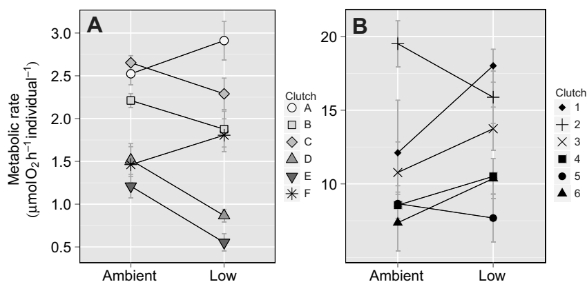
Fig. 2. Petrolisthes cinctipes oxygen consumption rate per brood of (A) embryos after 7–10 days exposure and (B) larvae after 4–10 days exposure to ambient pH (7.93±0.06) or low pH (7.58±0.06). Six separate broods were tested per stage (see key). Females used for hatching out larvae were different from those from which we obtained embryos. Each point represents the mean ± s.e.m. for N=4-10 individuals. *Significant difference ( P\leq 0.05 ) between pH treatments for a female's offspring within a developmental stage. Metabolic responses in embryos exhibited a significant interaction of pH treatment and brood (ANOVA, F_{9,91}=3.5 , P<0.0001 ).
