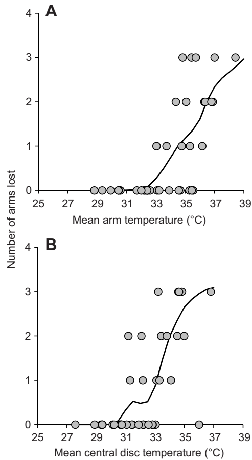
Fig. 4. Sublethal effects of temperature on Pisaster ochraceus . Number of arms lost in survivors as a function of their mean arm temperature (A) and mean central disc temperature (B). Curves illustrate the LOESS spline estimation from smoothed data with a tension of 0.40.
