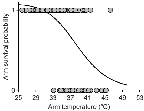
Fig. 5. Sublethal effects of temperature on Pisaster ochraceus . Survival probability of an arm when pooling all arms from survivors (1: intact arm, 0: arm loss) as a function of their temperature. The curve indicates the logistic dose–response regression model.
