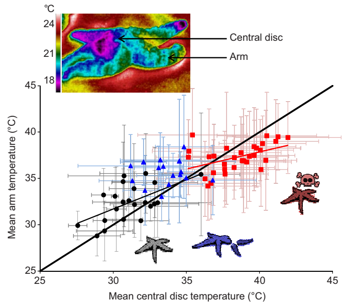
Fig. 1. Mean ( \pm s.d.) arm temperature as a function of mean ( \pm s.d.) central disc temperature for all Pisaster ochraceus individuals tested including the survivors with intact arms (black circles) and arm abscission (blue triangles), as well as the individuals that died (red squares). The linear regression lines are shown when correlations are significant. The black line indicates the equality of the two variables. The inset is an infrared image of a sea star during the exposure to experimental heating, illustrating the thermal heterogeneity of the sea star body surface (the color scale indicates temperature range).
