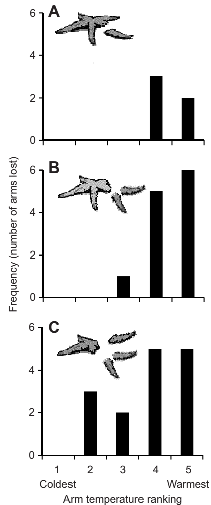
Fig. 6. Sublethal effects of temperature on Pisaster ochraceus . Temperature ranking of arm lost at the intra-individual scale (rank 1, coldest of the five arms, to rank 5, the hottest arm) for the groups that lost one (A), two (B) or three arms (C) after exposure to the heating treatment ( N=5 , 6 and 5 individuals in each group, respectively).
