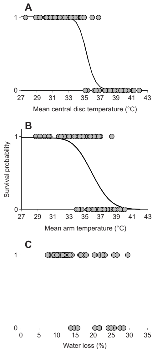
Fig. 3. Lethal effects of temperature on Pisaster ochraceus . Survival probability (1: survived, 0: died) of individuals according to mean central disc temperature (A) (from Pincebourde et al., 2008), mean arm temperature (B) and water loss (C). Curves indicate the logistic dose–response regression model.
