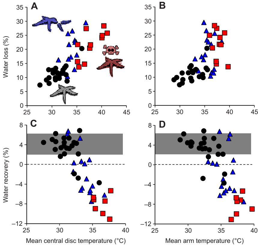
Fig. 2. Temperature influence on water balance in Pisaster ochraceus . (A,B) Water loss (% of initial wet body mass) during low tide as function of mean central disc temperature (A) and mean arm temperature (B). (C,D) Water recovery (% of initial wet body mass) during following high tide as function of mean central disc temperature (C) and mean arm temperature (D). The relationship is shown for survivors with no arm damage (black circles), survivors with arm abscission (blue triangles) and the individuals alive at the time of measurement that died subsequently (red squares). The gray bars indicate the expected water recovery portion ( 4.5 \pm 2.3\% of initial wet body mass; mean \pm s.d.) according to Pincebourde et al. (Pincebourde et al., 2009).
