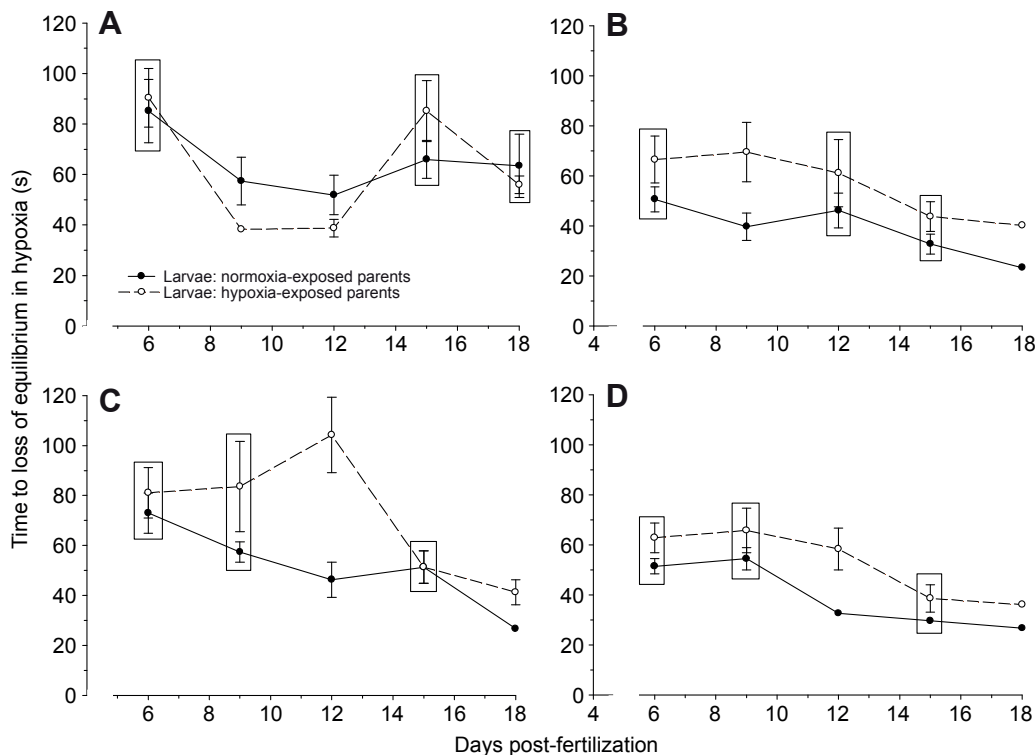
Fig. 5. Time to loss of equilibrium in hypoxia ( \sim 4 kPa O_2 ) of zebrafish of parents reared in normoxia or hypoxia for 1 (A; n=10 –23 per group), 2 (B; n=10 –14 per group), 3 (C; n=9 –14 per group) or 4 weeks (D; n=18 –29 per group). Points grouped within boxes are not significantly different from each other (two-way ANOVA with Tukey's post hoc analyses between treatment groups, P > 0.05 ). Mean values \pm 1 s.e.m. are presented.
