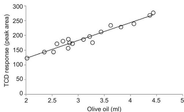
Fig. A2. Linear relationship between the volume of olive oil and amount of N_2 gas released. Points show the area of liberated N_2 peak from varying amounts of olive oil incubated with nitrogen gas; linear regression between the variables was significant ( P < 0.0001 ; R^2 = 0.94 ).
