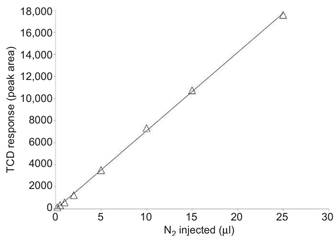
Fig. A1. Standard curve for injections of known amounts of N_2 . Points show the linear response of the thermal conductivity detector as a function of the amount of pure nitrogen gas injected into the gas chromatograph; the variables were highly correlated ( R^2 > 0.99 ).
