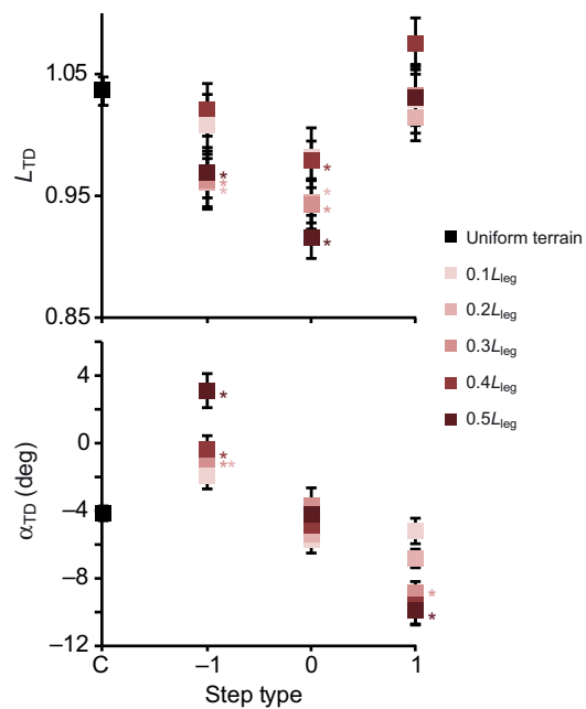
Fig. 4. Fractional effective leg length ( L_{\text{TD}} ) and velocity angle ( \alpha_{\text{TD}} ) at touchdown across step categories for all terrain conditions. Error bars indicate \pm s.e.m., revealing variation within terrain conditions, especially in L_{\text{TD}} . A consistent trend in \alpha_{\text{TD}} is observed with increasing obstacle height in steps '-1' and '1'. C, control (uniform terrain). Asterisks denote significant differences to uniform terrain.
