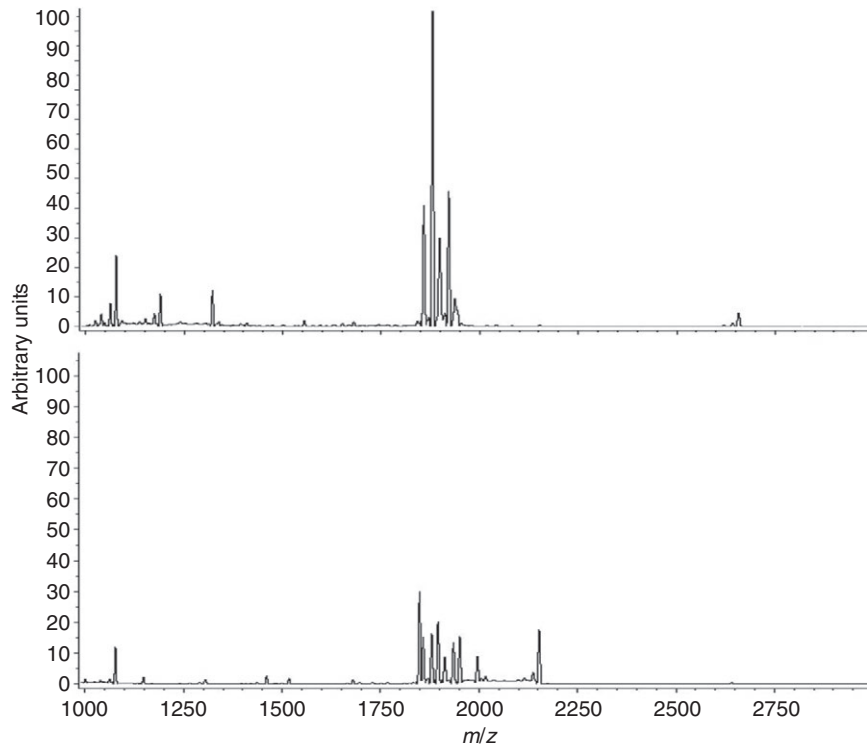
Fig. 3. CPC profiles of parasites (top) and host foundresses (bottom) in the pre-usurpation phase (two randomly chosen spectra are shown).
