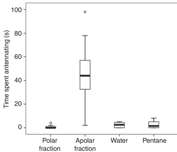
Fig. 1. Host nest detection response in the parasite is evoked by the nest hydrocarbons (apolar fraction). Parasites spent significantly more time antennating the apolar fraction than the polar fraction and the two controls (water and pentane). Box plots show medians (bold lines), the 75th and 25th percentiles (boxes), the extremes (vertical lines) and the outliers (circles).
