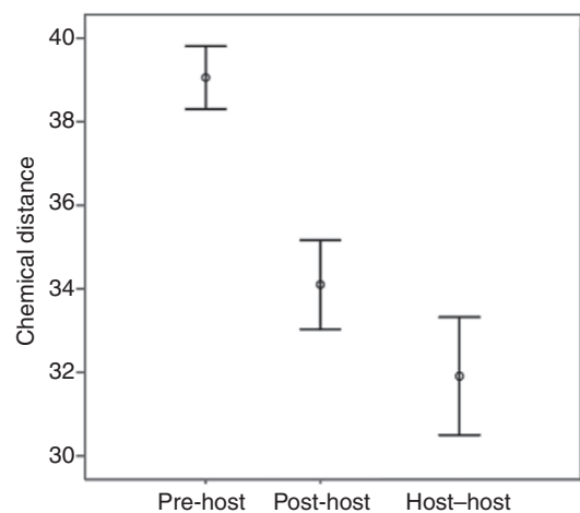
Fig. 4. The parasite CPC profile approaches that of the host after usurpation. The mean and the 95% confidence interval of the chemical distances between parasites and hosts before (pre-host) and after usurpation (post-host) and between two random hosts (host–host) are shown.
