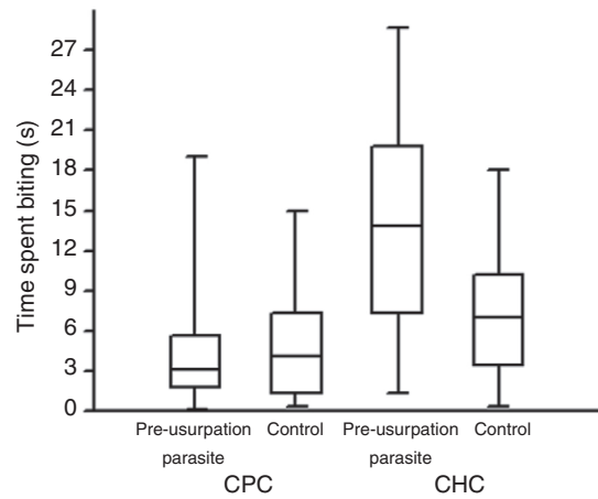
Fig. 2. Time spent biting the filter with the cuticular polar compound (CPC) extract of pre-urisdiction parasites and control (solvent) and the cuticular hydrocarbon (CHC) extract of pre-urisdiction parasites and control (solvent). Box plots show medians (bold lines), the 75th and 25th percentiles (boxes), the extremes (vertical lines) and the outliers (circles).
