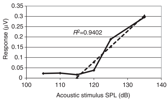
Fig. 6. Plot of the EFR amplitude at 1 kHz versus the corresponding acoustic stimulus sound pressure level (SPL) for the 150 kHz tone (solid line) and the linear regression (dashed line) calculated from 115 to 135 dB. The threshold was estimated as the intersection of the regression line with the zero value.
