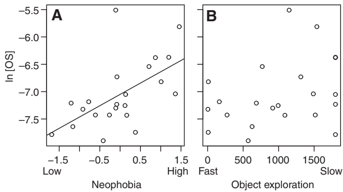
Fig. 3. Relationships between oxidative stress (OS; ROMs/OXY \times 1000) and personality traits. (A) Highly neophobic birds had higher OS than less neophobic birds. (B) No relationship was identified between OS and object exploration.
