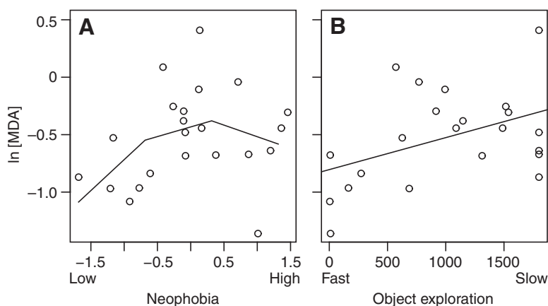
Fig. 4. Relationships between malondialdehyde (MDA; in \text{nmol ml}^{-1} ) and personality traits. (A) Birds with extremely high or low neophobia had lower MDA than intermediately neophobic birds. (B) Slow exploring birds had higher MDA than fast exploring birds.
