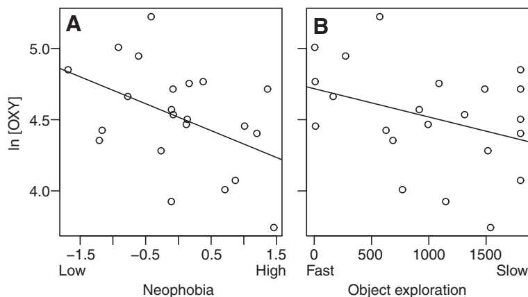
Fig. 2. Relationships between antioxidant capacity (OXY; in \text{mmol l}^{-1} of neutralised HOCl) and personality traits. (A) Highly neophobic birds had lower OXY than less neophobic birds. (B) Slow exploring birds had lower OXY than fast exploring birds.
