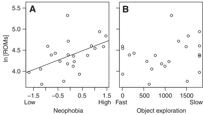
Fig. 1. Relationships between reactive oxygen metabolites (ROMs; in CARR U) and personality traits. (A) Highly neophobic birds had higher ROMs than less neophobic birds. (B) No relationship was identified between ROMs and object exploration.
