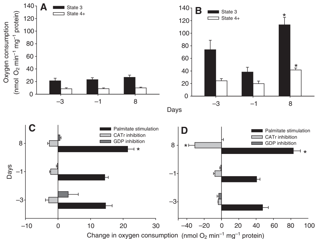
Fig. 1. Mitochondrial respiration rates and uncoupling (means \pm s.e.m.) in (A) liver and (B) skeletal muscle. State 3 (ADP-stimulated, black columns) and state 4+ (presence of oligomycin, white columns) rates were measured during development. ATP production (state 3) as well as the proton leak (state 4+) increased significantly 8 days after hatching in skeletal muscle but both parameters remained constant in liver. Mitochondrial uncoupling in (C) liver and (D) skeletal muscle in the presence of oligomycin stimulated by free fatty acid (addition of palmitate, black columns) significantly increased after hatching. In the presence of the ANT blocker carboxyatractylate (CATr), palmitate-stimulated oxygen consumption significantly decreased in liver and skeletal muscle (light grey columns). The proportion of ANT-induced mitochondrial uncoupling increased significantly 8 days after hatching in skeletal muscle but not in liver. Addition of the UCP blocker GDP (dark grey columns) had no effect in either tissue.
