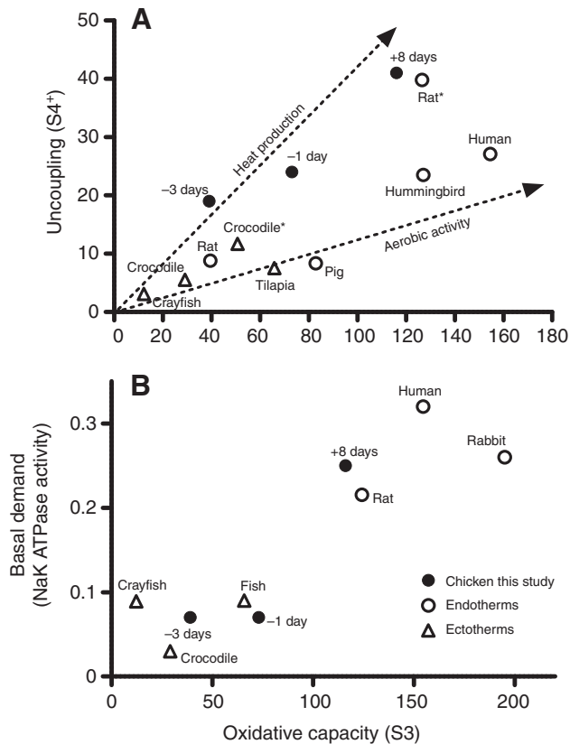
Fig. 5. Endothermy can be defined by the interactions between (A) metabolic capacity [here state 3 (S3) mitochondrial oxygen consumption ( \text{nmol mg}^{-1} \text{protein min}^{-1} )] and mitochondrial uncoupling [state 4 (S4+) mitochondrial oxygen consumption ( \text{nmol mg}^{-1} \text{protein min}^{-1} )] and (B) between metabolic capacity and cellular ATP demand [ \text{Na}^+/\text{K}^+ -ATPase activity ( \text{nmol P}_i \text{ min}^{-1} \text{g}^{-1} \text{ tissue} )]. Selection for increased aerobic activity would produce animals with high oxidative capacity and low uncoupling whereas selection for heat production would favour high oxidative capacity and high uncoupling (A). Mitochondrial oxygen consumption data are from Glanville and Seebacher (Glanville and Seebacher, 2006) for crocodile (crocodile=warm acclimated Crocodylus porosus ; crocodile*= C. porosus cold acclimated), E. J. Glanville and F.S. (unpublished data) for rat (rat=summer caught Rattus fuscipes ; rat*=winter caught R. fuscipes ); Schnell and Seebacher (Schnell and Seebacher, 2008) for the fish, tilapia ( Oreochromis mossambicus ); Seebacher and Wilson (Seebacher and Wilson, 2006) for crayfish ( Cherax destructor ); Suarez et al. [(Suarez et al., 1986) for hummingbird ( Selasphorus rufus ); Porta et al. (Porta et al., 2006) for pig; Willis and Jackman (Willis and Jackman, 1994) for rabbit; Tonkonogi and Sahlin (Tonkonogi and Sahlin, 1997) for human]. \text{Na}^+/\text{K}^+ ATPase data other than for chicken and humans (Fraser and McKenna, 1998) are from Else et al. (Else et al., 1996). Because of the paucity of tissue-specific data of \text{Na}^+/\text{K}^+ ATPase activities we matched activities of C. johnstoni with mitochondrial oxygen consumption of C. porosus (crocodile in B), Rattus norvegicus with Rattus fuscipes (rat), and Cyprinus carpio with Oreochromis mossambicus (fish).
