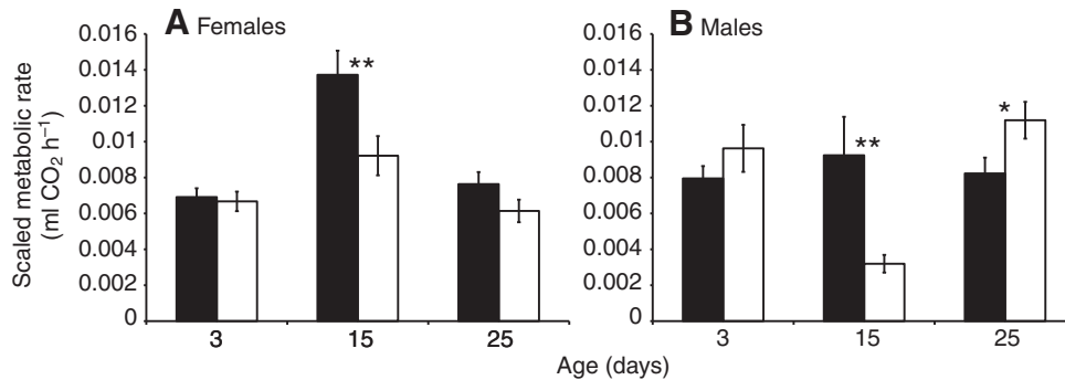
Fig. 3. Mean metabolic rate ( \pm s.e.m.) based on two 4 h windows (07:30–11:30 h and 11:30–15:30 h) for infected (black bars) and uninfected (white bars) males and females at three adult ages. Each bar represents data from 15 mosquitoes \times 3 replicates \times 2 windows. * P <0.05, ** P <0.01.
