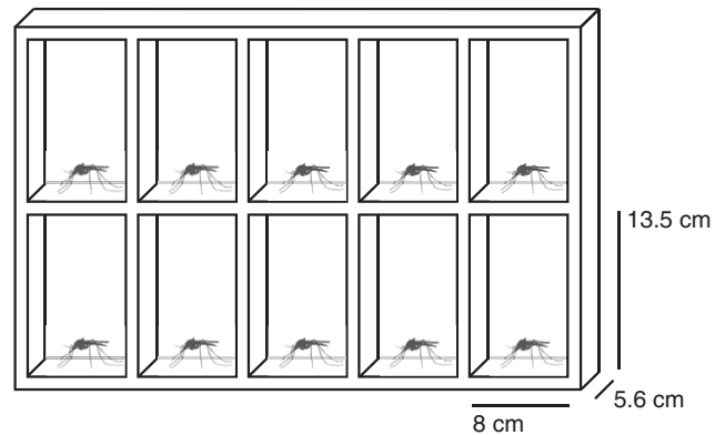
Fig. 1. Mosquito observation chamber with 10 individual cells constructed with white opaque plastic. Cells are covered with a sliding door of transparent plastic for videography.
