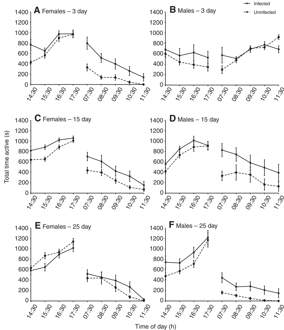
Fig. 2. Mean total time active ( \pm s.e.m.) per 1 h window for infected and uninfected males and females at three adult ages. Times on x-axis denote the beginning of the hour-long session. Lights were turned on daily at 07:00 h and off at 19:00 h. Each point represents 10 mosquitoes \times 3 replicate recording days.
