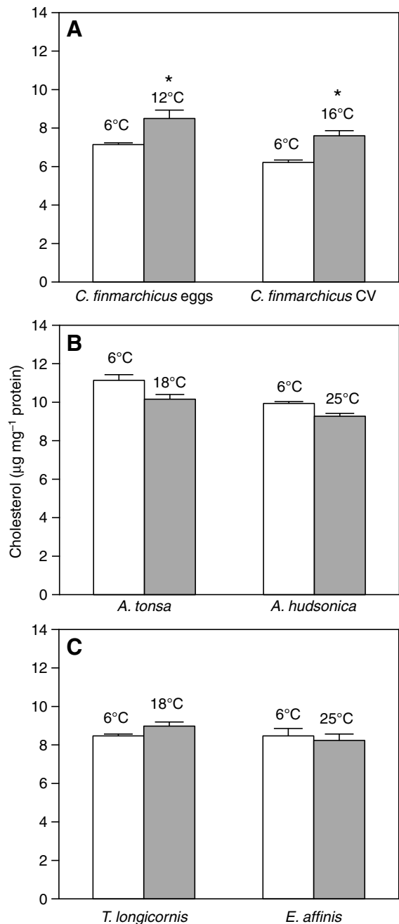
Fig. 1. Effect of acclimation to warm and cold temperatures on cholesterol content of Calanus finmarchicus eggs and CV copepodites (A), Acartia hudsonica and Acartia tonsa (B), Temora longicornis and Eurytemora affinis (C). Acclimation temperatures are given above columns. Data are means \pm s.e.m. *Significant difference at P < 0.05 (two-way ANOVA). Sample sizes (number of replicate containers per incubator) for each species are: C. finmarchicus , N=6 (eggs), N=8 (copepodites), A. hudsonica , N=2 ; A. tonsa , N=2 ; T. longicornis , N=6 ; E. affinis , N=10 . One subsample was taken per replicate container except for Acartia spp., for which four subsamples were taken.
