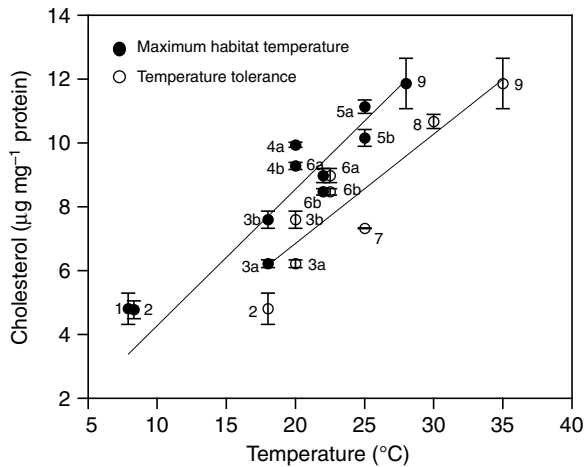
Fig. 3. Relationship between cholesterol content and habitat temperature in copepods. Cholesterol content ( \mu\text{g cholesterol mg}^{-1}\text{ protein} ) plotted against both maximum habitat temperature (filled circles) and temperature tolerance based on \text{LD}_{50} (open circles). Species identifications given adjacent to markers: (1) Euchaeta norvegica , (2) Calanus glacialis , (3a) Calanus finmarchicus cold acclimated, (3b) C. finmarchicus warm acclimated, (4a) Acartia hudsonica cold acclimated, (4b) A. hudsonica warm acclimated, (5a) Acartia tonsa cold acclimated, (5b) A. tonsa warm acclimated, (6a) Temora longicornis cold acclimated, (6b) T. longicornis warm acclimated, (7) Centropages hamatus , (8) Centropages typicus , (9) Eurytemora affinis . To conform to the conditions experienced by the other copepods, E. affinis was acclimated to seawater (32 p.p.t.) for 7 days. Data are presented as mean \pm s.e.m. Sample sizes are N=10 for E. norvegica , C. typicus and E. affinis ; N=8 for C. finmarchicus , N=6 for C. glacialis and T. longicornis , and N=2 for A. hudsonica , A. tonsa , and C. hamatus . Correlation analysis of temperature tolerance, r^2=0.82 , significance level P<0.001 , maximum habitat temperature r^2=0.84 , significance level P<0.001 .
