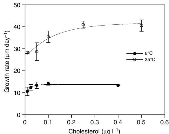
Fig. 2. Growth rates of the copepod Eurytemora affinis at 6°C and 25°C at different concentrations of dietary cholesterol. Two replicates were used per treatment, with each replicate calculated from the average length of 45–90 nauplii or copepodites. Data are presented as means \pm s.e.m.
