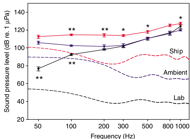
Fig. 3. Mean ( \pm s.e.m.) hearing thresholds of the Lusitanian toadfish under laboratory conditions (baseline; black line) and in the presence of ambient noise (blue line) and ship noise (red line). Dashed lines of same colour show the cepstrum-smoothed sound power spectra for the respective noise types used during audiogram determinations. Asterisks indicate statistically significant differences between the ambient noise and baseline (unpaired t -tests) as well as ambient and ship noise (paired t -tests); * P<0.007 and ** P<0.001 ). N=9 , baseline; N=6 , ambient and ship noise audiograms.
