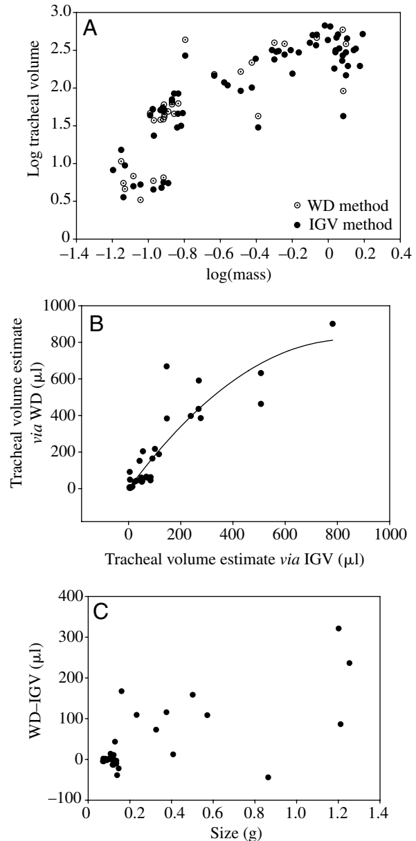
Fig. 4. Water displacement (WD) method and inert gas volumetric (IGV) method comparisons. (A) Both methods predict a similar increase in tracheal volume with mass. (B) Estimate of tracheal volume using the WD method versus IGV method for the same individuals. (C) The difference between the tracheal volume estimates using the WD method versus the IGV method as a function of body size. The WD method predicted larger tracheal volumes than the IGV method, with absolute difference increasing with animal size.
