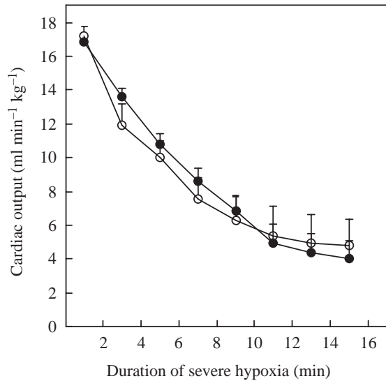
Fig. 3. Cardiac output ( \dot{Q} ) during 15 min of severe hypoxia (filled circles; N=8 ), and during 15 min of severe hypoxia with 1.5 \text{ mmol l}^{-1} of sodium cyanide (NaCN) added to the hypoxic perfusate (open circles; N=7 ). \dot{Q} was averaged over 2 min intervals during severe hypoxia. There was no significant difference in \dot{Q} between the treatment groups, at any point during severe hypoxia.
