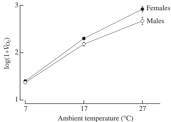
Fig. 2. Interaction plot (see Table 2) from an ANCOVA, with body mass M_b as the covariate, showing the relationship between sex and ambient temperature T_a on \dot{V}O_2 . Data were transformed to \log+1 to meet ANOVA assumptions. Values are adjusted means \pm S.E.M. ( N=75 , 147 and 70 for 7°C, 17°C and 27°C, respectively).
