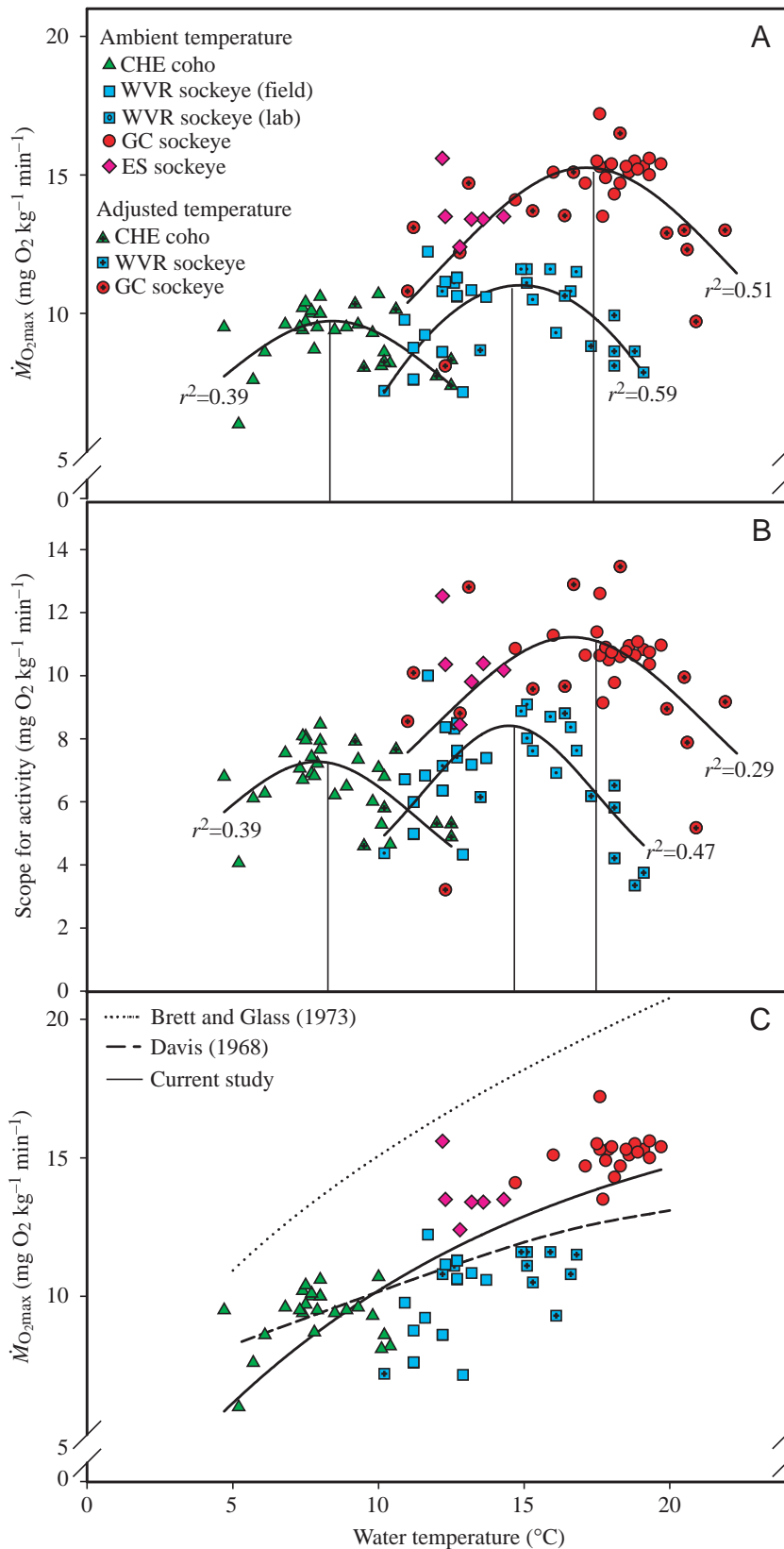
Fig. 3. (A) Stock-specific relationships between oxygen consumption at U_{\text{crit}} ( \dot{M}_{O_2\text{max}} ) and water temperature t from different fish stocks (GC, Gates Creek stock; WVR, Weaver Creek stock; CHE, Chehalis River stock; ES, Early Stuart stock). Fish were tested at either ambient temperature (symbols without a cross) or an adjusted temperature (symbols with a cross). The vertical lines indicate the average ambient water temperature for each stock, which corresponded closely with the peak \dot{M}_{O_2\text{max}} for that stock. For GC sockeye salmon: \dot{M}_{O_2\text{max}}=15.26/1+[(t-17.13)/8.95]^2 ( P<0.05 ; r^2=0.51 ). For WVR sockeye salmon: \dot{M}_{O_2\text{max}}=-100.82+119.2/1+[(t-14.88)/25.52]^2 ( P<0.05 ; r^2=0.59 ). For CHE coho salmon: \dot{M}_{O_2\text{max}}=9.72/1+[(t-8.42)/7.31]^2 ( P<0.05 ; r^2=0.39 ). (B) Stock-specific relationships between scope for activity ( \dot{M}_{O_2\text{max}}-\dot{M}_{O_2\text{routine}} ) and water temperature from different fish stocks. The vertical lines indicate the average ambient water temperature for each stock, which corresponded closely with the peak \dot{M}_{O_2\text{max}} for that stock. For GC sockeye salmon: scope for activity= 11.22/1+[(t-16.63)/8.11]^2 ( P<0.05 ; r^2=0.29 ). For WVR sockeye salmon: scope for activity= 7.29/1+[(t-7.89)/6.03]^2 ( P<0.05 ; r^2=0.47 ). For CHE coho salmon: scope for activity= 8.41/1+[(t-14.48)/5.10]^2 ( P<0.05 ; r^2=0.39 ). (C) Relationship between \dot{M}_{O_2\text{max}} and ambient water temperature among individual fish from different stocks of sockeye and coho salmon. The regression equation for the relationship (solid line, P<0.05 ; r^2=0.63 ) is compared with earlier studies of adult sockeye salmon (broken line, Davis 1966; dotted line, Brett and Glass, 1973).
