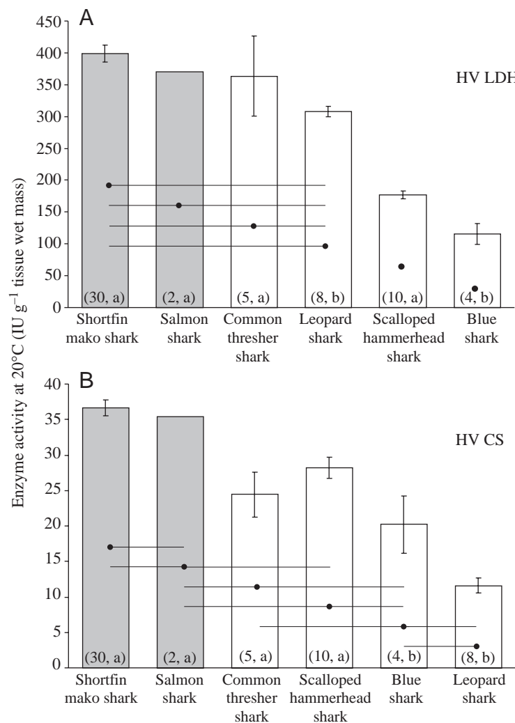
Fig. 2. (A) Lactate dehydrogenase (LDH) and (B) citrate synthase (CS) activities at 20°C in shark heart ventricle (HV; an unknown mixture of compact and spongy myocardium). Values are means \pm S.E.M. for ectothermic sharks (open bars) and sharks known to be endothermic (shaded bars). Values in parentheses at the base of each bar are the sample size and the data source: a, present study; b, Dickson et al. (1993). Horizontal lines group species that do not differ significantly from the comparison species (indicated by a black circle), as determined by a Tukey–Kramer multiple comparisons test at P < 0.05 . For example, leopard shark HV CS (bottom horizontal line in B) is not significantly different from that of the blue shark but differs significantly from all other species studied.
