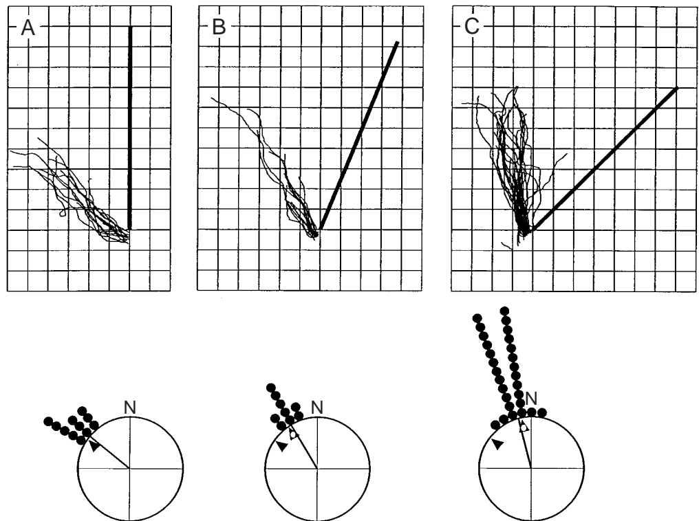
Fig. 2. Homeward paths of ants caught near the nest (as in Fig. 1C) and then carried to a point on the test field close to the end of the barrier. Paths are shown beginning where the ants are in line with barrier. (A) Barrier oriented as in training; (B) barrier rotated clockwise through 22^\circ ; (C) barrier rotated clockwise through 45^\circ . In this and the remaining figures, the circular histogram below each set of trajectories shows the direction of each trajectory that was 3 m or longer, with the mean direction of the trajectories being drawn as a radius. Here, and in Fig. 4, the filled triangles show the direction of the nest from the end of the barrier and the open triangle shows the bearing of that direction plus the angle through which the barrier was rotated. N, north.
