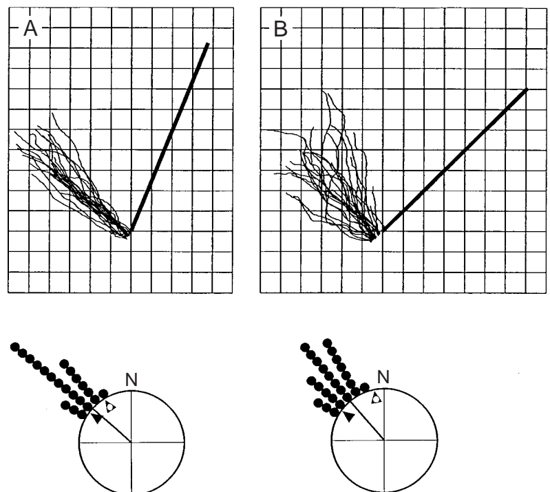
Fig. 4. Homeward paths of ants caught at the feeder and taken to a point on the test field close to the end of the barrier. (A) Barrier rotated clockwise through 22^\circ ; (B) barrier rotated through clockwise 45^\circ . For further details, see Fig. 3. N, north.
