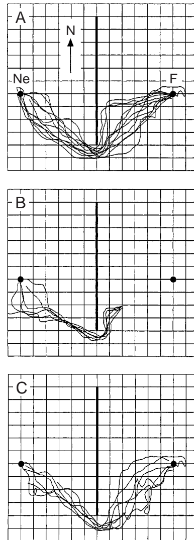
Fig. 1. Homeward paths of ants detouring around a familiar barrier to reach their nest. (A) Uninterrupted paths of ants from a familiar feeder to the nest. (B) Trajectories of ants taken from the feeder to a point 2 m to the east and 2 m to the north of the southern tip of the barrier. (C) Trajectories of ants allowed to return to within 1 m of the nest before being captured and replaced at the feeder. In this and subsequent figures, the barrier is shown by the thickened vertical line. Ne and F indicate nest and feeder respectively. The spacing between grid lines is 1 m. N, north.
