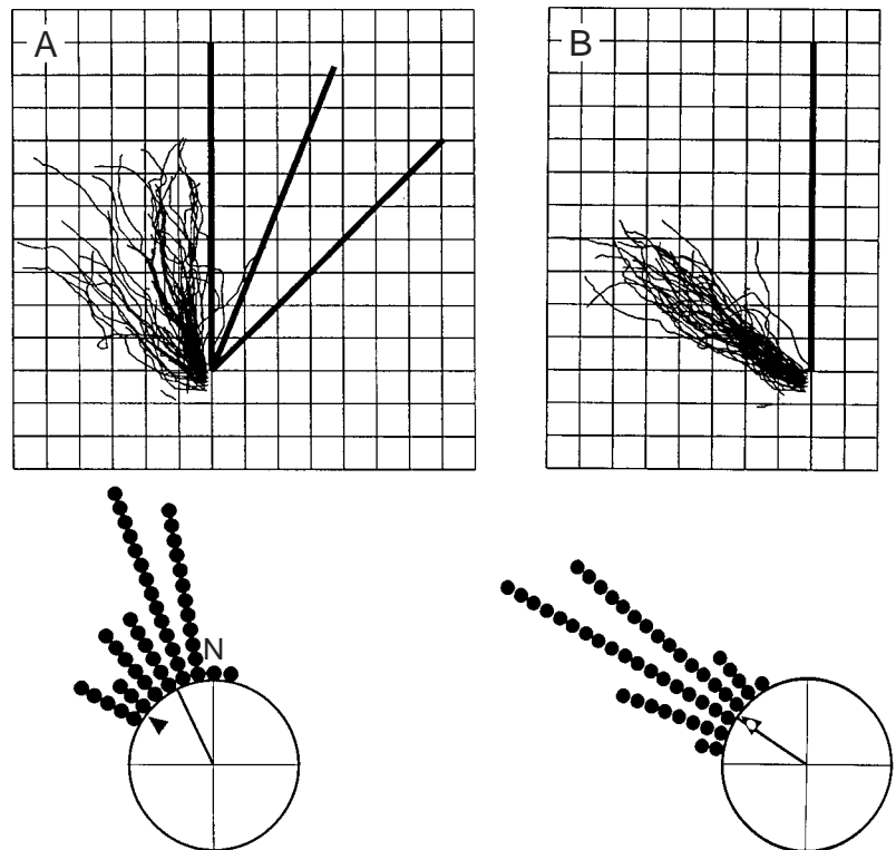
Fig. 3. Trajectories from Fig. 2 superimposed. (A) Superimposition without rotation. The filled triangle shows the direction of the nest from the end of the barrier. (B) Trajectories rotated by 0, 22 or 45^\circ so as to align the barriers. The open triangle shows the predicted direction assuming that the trajectories are controlled by visual cues from the barrier. N, north.
