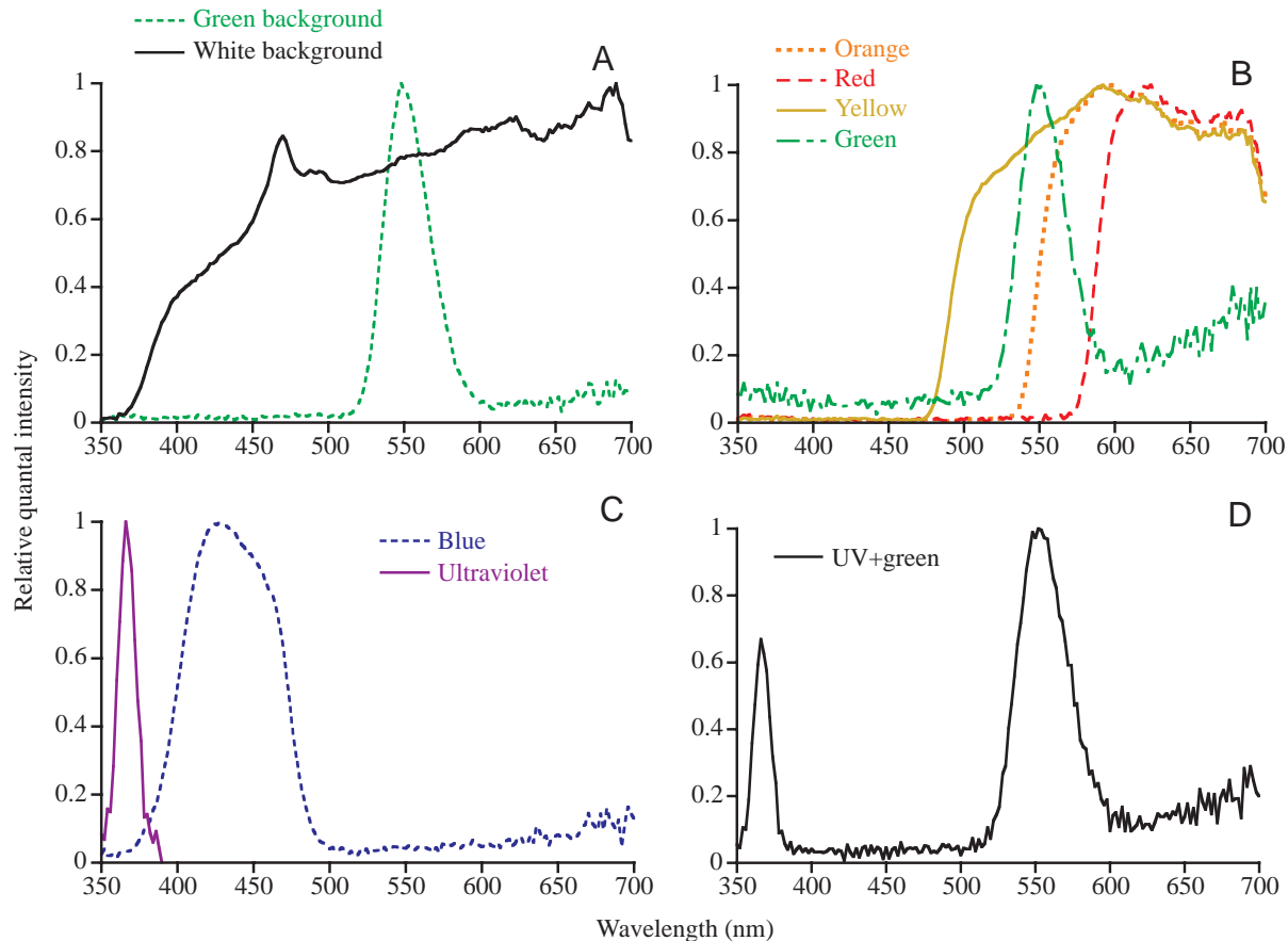
Fig. 4. The spectral radiance of each stimulus and background used in the experiments was measured using a radiance probe attached to the fibre-optic input of an Ocean Optics PS1000 fibre-optic spectroradiometer. The radiance probe was placed where the lizards sat during the experiment. Prior to each measurement, a test light was passed out through the radiance probe to identify the precise sampling location. Each spectrum is shown relative to its peak value. The intensities of different spectra were adjusted using spectrally flat neutral density filters that altered the intensity at all wavelengths equally. (A) The two background spectra employed in the different experiments. The 'green' background was created with a Kodak Wratten filter no. 99 (550 nm peak transmittance). The 'white' background was created without colour filters. Neutral density filters were used with both background spectra to make them equal in estimated brightness. The total radiance of the green background was 0.029 \mu\text{mol m}^{-2} \text{s}^{-1} \text{sr}^{-1} (where 1 \mu\text{mol} = 6.02 \times 10^{17} photons), and the radiance of the white background was 0.053 \mu\text{mol m}^{-2} \text{s}^{-1} \text{sr}^{-1} , which was calculated to have an estimated brightness equal to that of the green background. (B) The stimulus flag spectra used in experiment 2. The four spectra used were referred to as green, yellow, orange and red on the basis of their appearance to a human observer. The green stimulus spectrum was created with a Kodak Wratten filter no. 99. The other spectra were created with glass long-pass colour filters (Oriel) with cut-on wavelengths at 495 nm (yellow), 550 nm (orange) and 590 nm (red). Neutral density filters were mounted with each colour filter to adjust them to equal brightness. They were set to be nearly equal in estimated brightness to the background at the middle intensity setting on the variable neutral density filter. (C) Spectra of the stimulus flags employed in experiment 2. The green background from (A) and the green stimulus from (B) were also employed in this experiment. The ultraviolet stimulus was created with an Oriel UV interference filter with a peak at 360 nm, while the blue stimulus was created with an Oriel glass bandpass filter with a peak at 420 nm. (D) The spectrum of the stimulus flag used in experiment 3. The green portion was created with a Kodak Wratten filter no. 99, and the ultraviolet (UV) portion was created with an ultraviolet interference filter. The two components were combined as shown in Fig. 3B.
