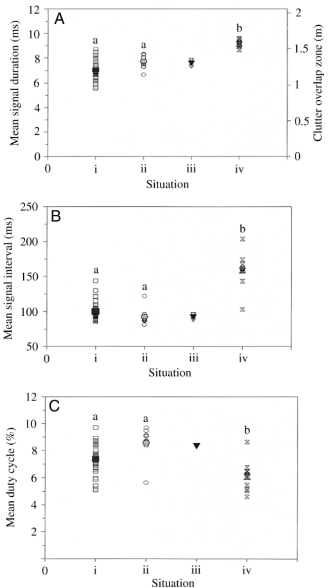
Fig. 1. Mean signal duration (A), signal interval (B) and duty cycle (C) for searching signals recorded from bats in four situations: (i) flying above the hay field searching for Hepialus humuli , (ii) prior to an attack on a H. humuli , (iii) just prior to capture of H. humuli , and (iv) as in i, except that the bat was searching for other insects above a road. Open symbols are means of sequences, and filled symbols are the overall mean for each situation. Different letters indicate a significant difference ( P < 0.005 ) between situations. No letters are given for situation iii because of the low value of N (see text for explanation).
