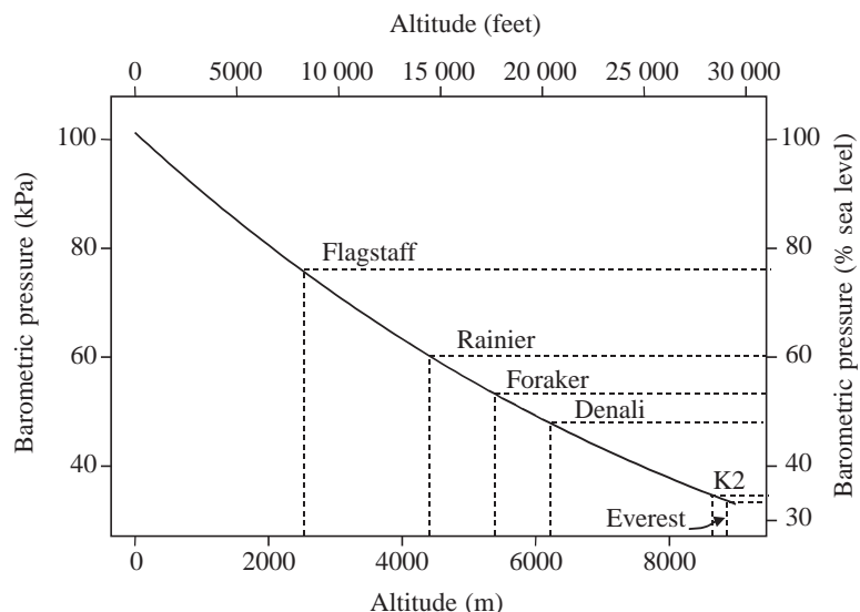
Fig. 1. Barometric pressure as a function of altitude. The left-hand ordinate plots absolute pressure in kPa and the right-hand one scales pressure as a percentage of sea-level value. The solid curve is calculated from West (West, 1998). Dashed lines connect altitudes and estimated relative barometric pressures of various localities or summits.
