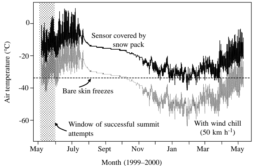
Fig. 2. Temperatures at the South Col (7891 m) of Everest from May 1999 to May 2000. The upper line plots measured air temperatures (data courtesy M. Hawley and the MIT Media Group). The lower line plots estimated wind chill, assuming a wind speed of 50 \text{ km h}^{-1} (see text). The period over which successful ascents of Everest occurred in 1999 is shaded.
