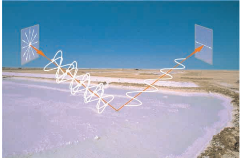
Fig. 2. Polarization arising from the reflection of light by a water surface. Unpolarized sunlight (left panel) becomes linearly polarized when it is reflected by water surfaces. The reflected light is horizontally polarized (right panel). Maximum polarization is reached at a particular angle of incidence (Brewster's angle; 53^\circ for the air/water interface). Background landscape: Sabkhat al Muh, south-east of Tadmur, Syria.
