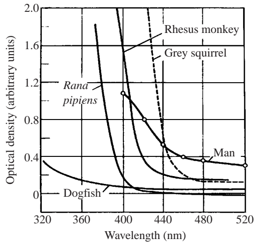
Fig. 1. The spectral absorbance of ocular filters in the eyes of various vertebrates. (Redrafted from Muntz, 1972, with the permission of Springer-Verlag and W. R. A. Muntz.)
