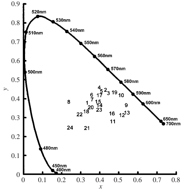
Fig. 4. Plots of 24 coloured stimuli (numbered as in Table 1) in CIE 1931 colour space. The chromaticity coordinates (x, y) of the stimuli are plotted considering an illumination of correlated colour temperature=6500 K, and the spectral locus is a plot of pure spectral radiation.
