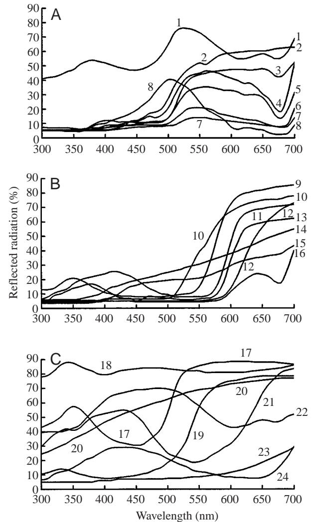
Fig. 2. Reflectance spectra of the 24 stimuli (numbered 1–24) described in Table 1. Division of the stimuli into A, B and C is purely to aid the reading of the reflectance curves.
