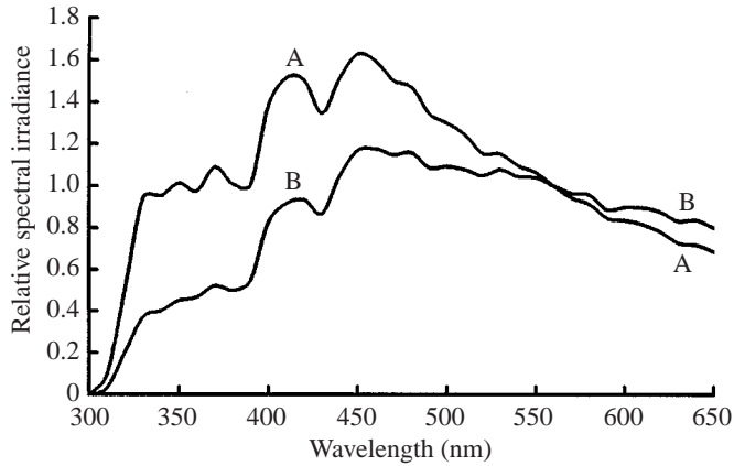
Fig. 3. Spectral distribution of typical daylight with the relative quantity of radiation normalised to 1.0 at 560 nm. Curves are based on the data of Judd et al. (Judd et al., 1964) and represent correlated colour temperatures of (A) 10 000 K and (B) 6500 K.
