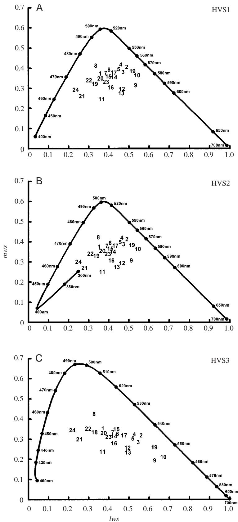
Fig. 6. Plots of 24 coloured stimuli (numbered as in Table 1) onto Cartesian coordinates to represent the colour space of various hypothetical visual systems (HVSs) considering an illumination of correlated colour temperature=6500 K. Chromaticity coordinates ( lws , mws ) are the normalised stimulations of the long-wavelength-sensitive and medium-wavelength-sensitive photoreceptors. (A) Colour space for HVS1, which is a visual system based on human colour receptor peaks (420, 534 and 564 nm; Bowmaker and Dartnall, 1980) and ocular filters absorbing radiations shorter than 400 nm. (B) Colour space for HVS2, which is a visual system based on human colour receptor peaks and no ocular filters. Ultraviolet radiation is assumed to be absorbed by secondary \beta -band peaks that are maximally sensitive to 340 nm radiation. (C) Colour space for HVS3, which is a visual system based on symmetrically spaced photoreceptors maximally sensitive at 420, 492 and 564 nm and assumes that all radiations shorter than 400 nm are absorbed by ocular filters (see Fig. 5). The spectral locus is a plot of pure spectral radiation.
