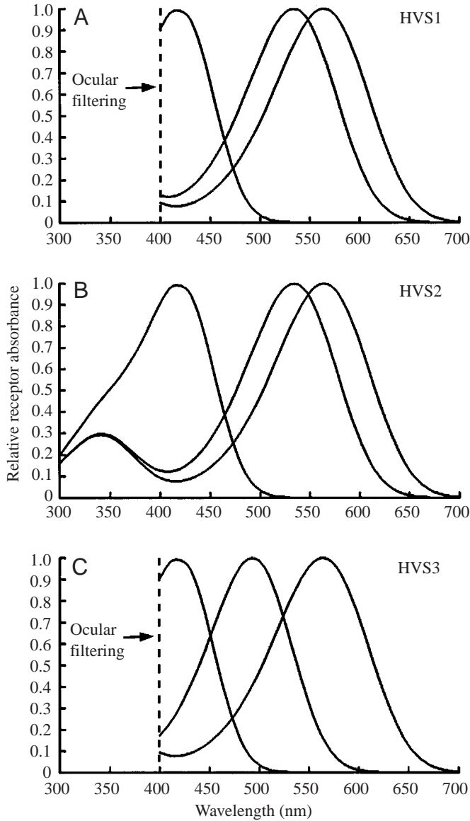
Fig. 5. Spectral sensitivity of various hypothetical visual systems (HVSs) plotted using a vitamin A 1 template described by Stavenga et al. (Stavenga et al., 1993) with the height of the photoreceptors adjusted to a maximum of 1.0. (A) HVS1 is based on human photoreceptor peaks at 420, 534 and 564 nm (Bowmaker and Dartnall, 1980) and assumes that all radiations shorter than 400 nm are absorbed by ocular filters. (B) HVS2 is based on the same photoreceptor peaks as HVS1, but assumes no ocular filtration and that ultraviolet radiations are absorbed by common \beta -band peaks maximally sensitive at 340 nm. (C) HVS3 is based on three symmetrically spaced photoreceptors maximally sensitive at 420, 492 and 564 nm and assumes that all radiations shorter than 400 nm are absorbed by ocular filters.
