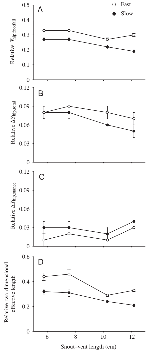
Fig. 4. Mean relative (divided by snout-vent length) values of hip height Y_{\text{hip}} at footfall (A), total change in Y_{\text{hip}} for the entire stride cycle (B), change in Y_{\text{hip}} during stance (C) and two-dimensional effective limb length at footfall (D). Values are means \pm S.E.M. Table 3 summarizes significant differences among size classes and speeds. Some of the standard errors are smaller than the symbols. Open and filled symbols represent fast ( 250\text{ cm s}^{-1} ) and slow ( 50\% duty factor) locomotion, respectively.
