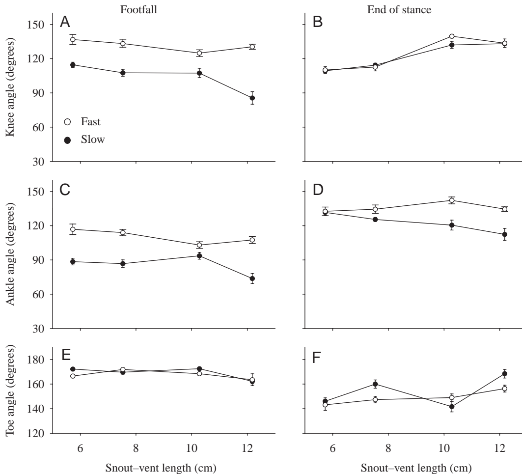
Fig. 6. Mean values of joint angles for the knee (A,B), ankle (C,D) and toe (E,F) at footfall (A,C,E) and at the end of stance (B,D,F). Values are means \pm S.E.M. Table 4 summarizes significant differences among size classes and speeds. Some of the standard errors are smaller than the symbols. Open and filled symbols represent fast (250 cm s -1 ) and slow (50% duty factor) locomotion, respectively.
