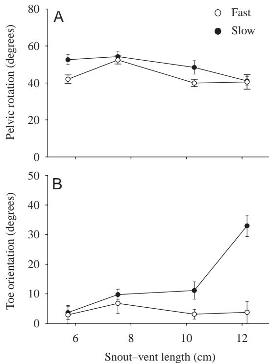
Fig. 9. Mean values of pelvic rotation (A) and the angle of toe orientation (B). Values are means \pm S.E.M. Table 5 summarizes significant differences among size classes and speeds. Open and filled symbols represent fast (250 cm s -1 ) and slow (50% duty factor) locomotion, respectively.
