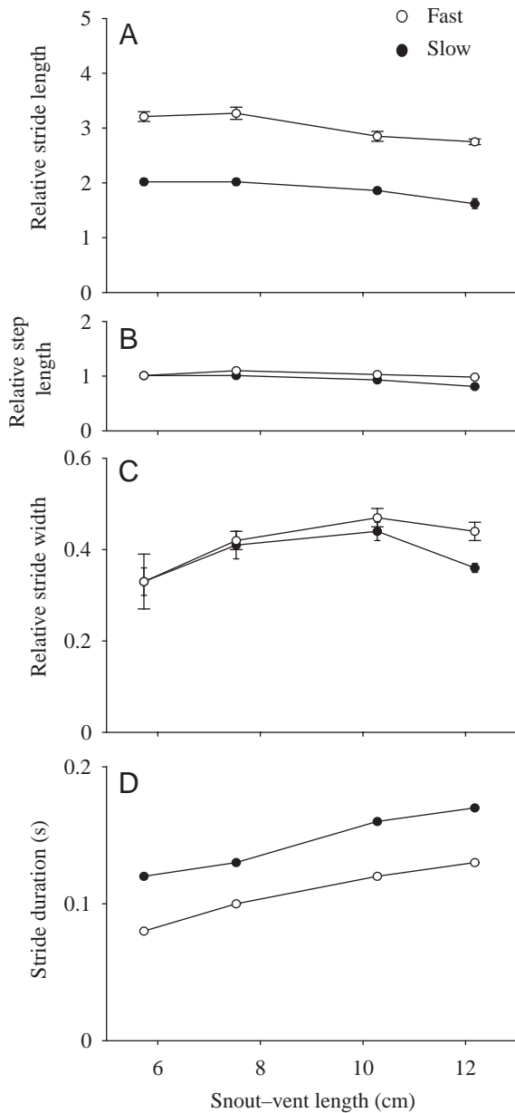
Fig. 3. Mean values of relative (divided by snout-vent length) stride length (A), relative step length (B), relative stride width (C) and stride duration (D) versus mean snout-vent length. Open and filled symbols represent fast ( 250\text{ cm s}^{-1} ) and slow ( 50\% duty factor) locomotion, respectively. Table 3 summarizes significant differences among size classes and speeds. Values are means \pm S.E.M. Some of the standard errors are smaller than the symbols.
