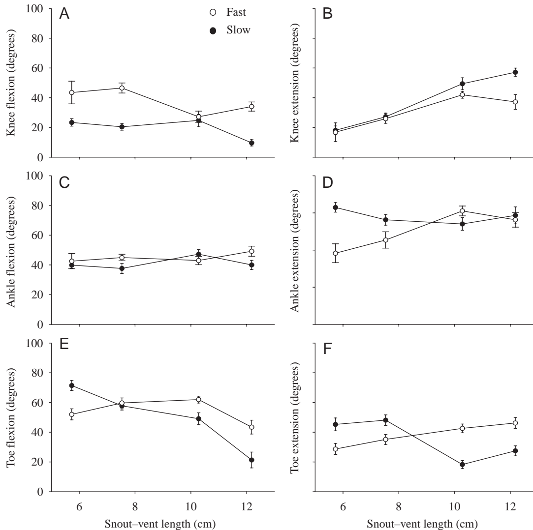
Fig. 7. Mean values of flexion (A,C,E), and extension (B,D,F) for the knee (A,B), ankle (C,D) and toe (E,F) during stance. Values are means \pm S.E.M. Table 4 summarizes significant differences among size classes and speeds. Open and filled symbols represent fast ( 250 \text{ cm s}^{-1} ) and slow ( 50\% duty factor) locomotion, respectively.
