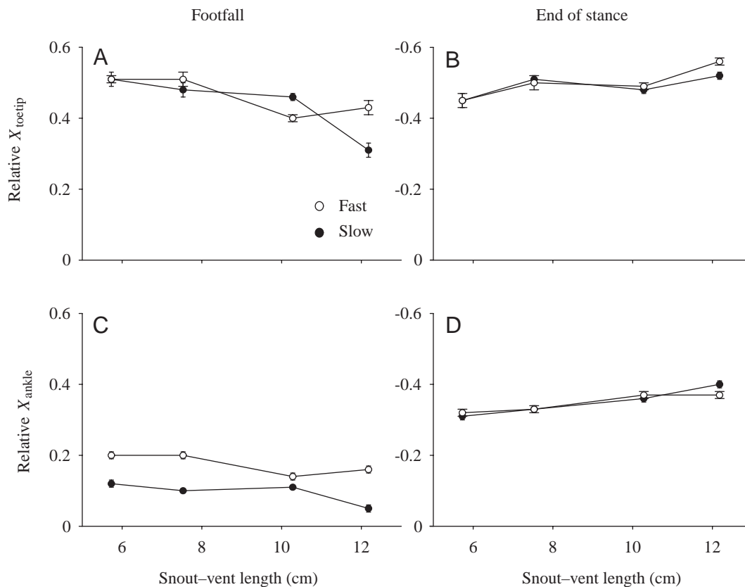
Fig. 5. Mean relative (divided by snout–vent length) values of the anterior–posterior position of the toe tip X_{\text{toetip}} (A,B), and ankle X_{\text{ankle}} (C,D) at footfall (A,C) and at the end of stance (B,D). Values are means \pm S.E.M. Table 3 summarizes significant differences among size classes and speeds. Some of the standard errors are smaller than the symbols. Open and filled symbols represent fast ( 250 \text{ cm s}^{-1} ) and slow (50% duty factor) locomotion, respectively.
