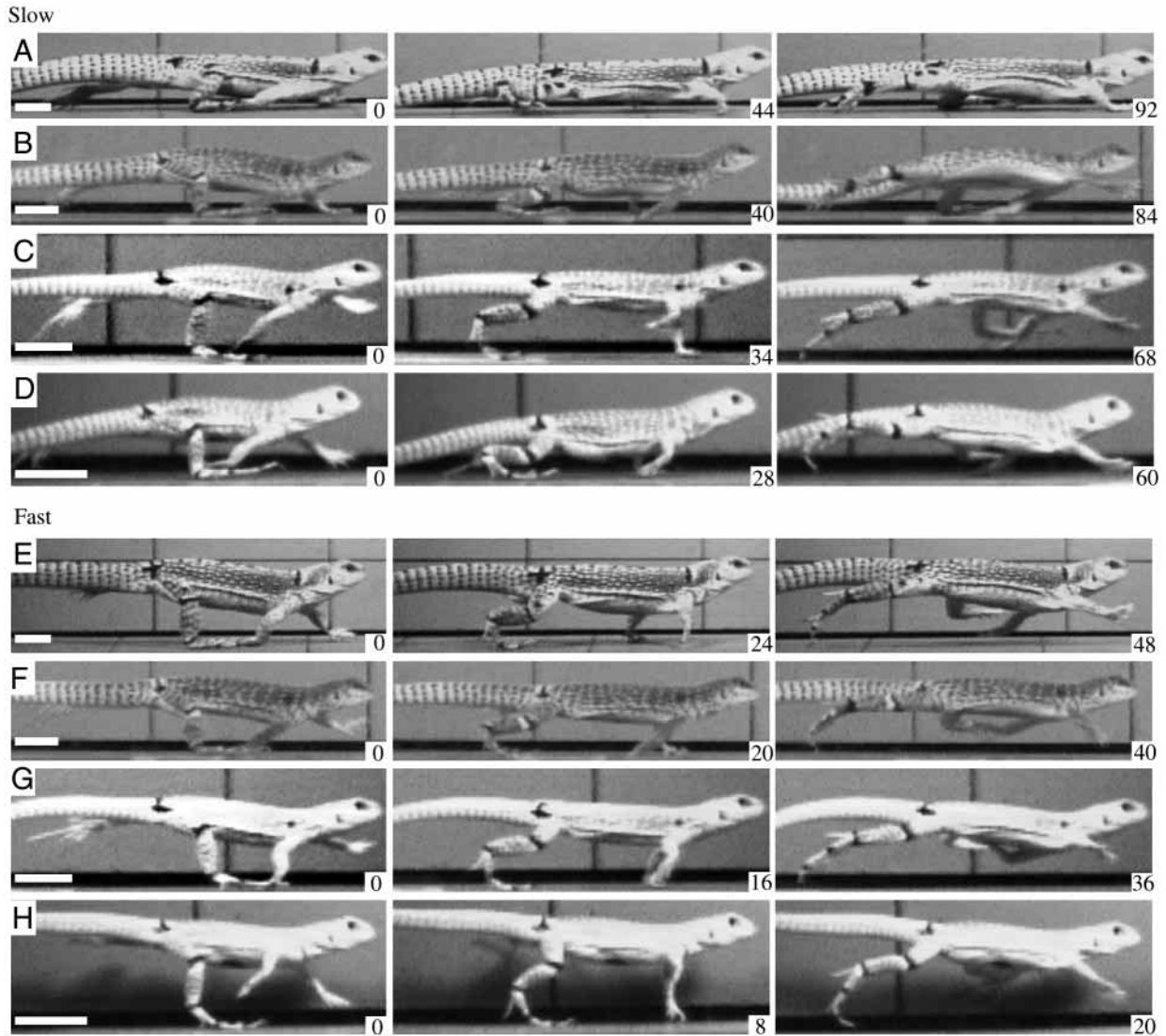
Fig. 2. Representative lateral views of single adult (A,E) (snout–vent length, SVL 11.9 cm, mass 59.5 g), subadult (B,F) (SVL 9.8 cm, mass 26.1 g), intermediate (C,G) (SVL 7.7 cm, mass 11.8 cm) and juvenile (D,H) (SVL 5.9 cm, mass 6.8 g) Dipsosaurus dorsalis with approximate duty factors and speeds of 50% (A–D) and 250 \text{ cm s}^{-1} (E–H), respectively. The three images within each row are at the times of footfall (left), mid-stance (centre) and the end of stance (right). Scale bars, 2 cm. The elapsed times after footfall (ms) are indicated in the lower right-hand corners. Video recordings of the locomotion of D. dorsalis can be found at http://www.biology.uc.edu/faculty/jayne/videos.htm .
