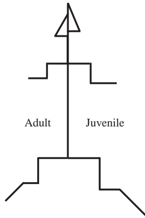
Fig. 1. A stick figure showing the average head and limb dimensions of a juvenile (snout–vent length, SVL 5.7 cm) and adult (SVL 12.2 cm) Dipsosaurus dorsalis scaled to the same trunk length. From proximal to distal, the line segments within the forelimb are the humerus, ulna and forefoot, and those of the hindlimb are the femur, tibia, tarsals+metatarsals and fourth toe.
