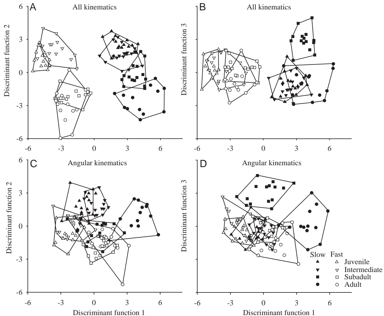
Fig. 10. Discriminant functions 2 and 3 versus discriminant function 1 from two separate analyses of a total of 20 relative linear, timing and angular variables (A,B) and a total of 14 angular variables (C,D). Circles, squares, upside-down triangles and right-side-up triangles represent individual strides of adult, subadult, intermediate and juvenile Dipsosaurus dorsalis , respectively. Table 6 provides loadings for both discriminant function analyses. Open and filled symbols represent fast ( 250 \text{ cm s}^{-1} ) and slow ( 50\% duty factor) locomotion, respectively.
