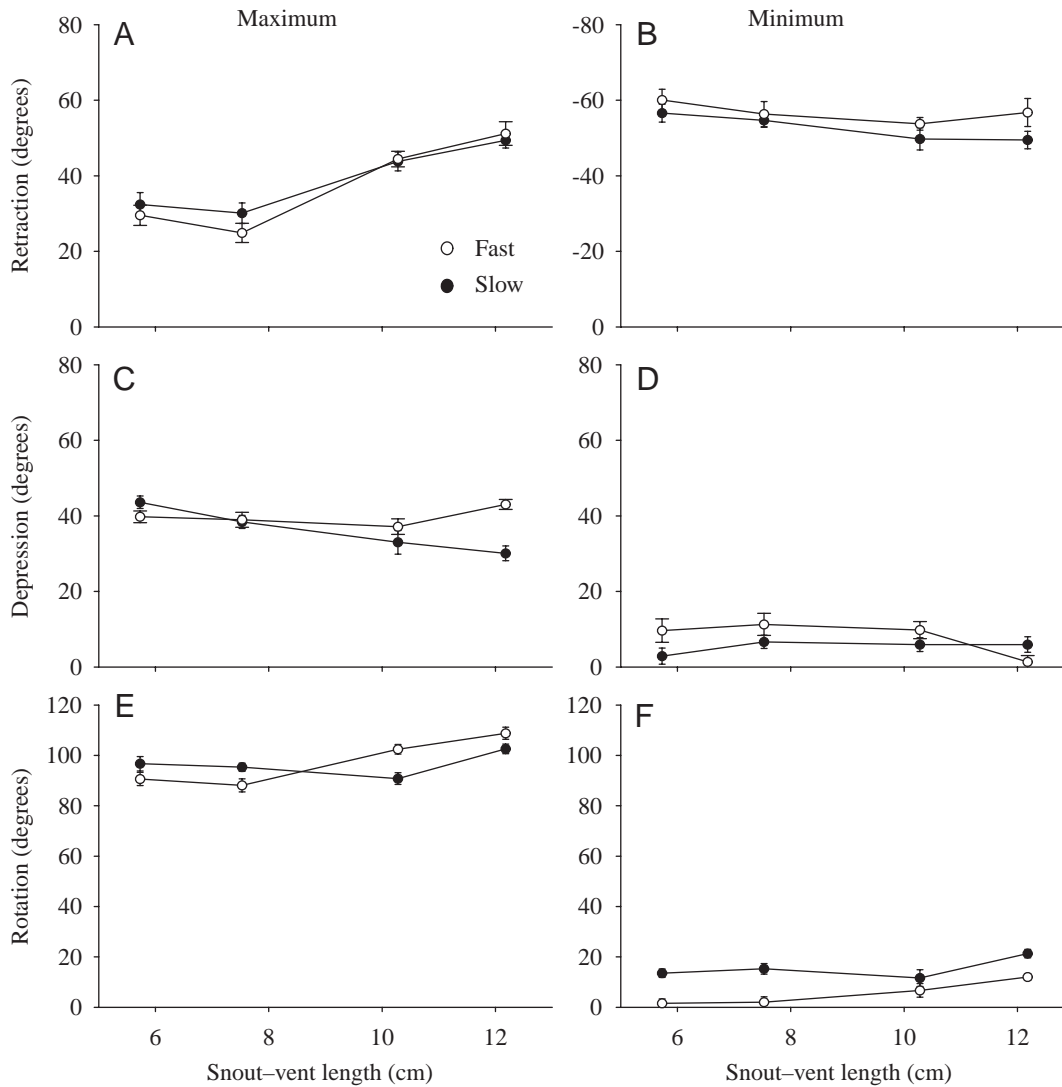
Fig. 8. Mean maximum (A,C,E) and minimum (B,D,F) values of retraction (A,B), depression (C,D) and rotation (E,F) of the femur. Values are means \pm S.E.M. Table 5 summarizes significant differences among size classes and speeds. Some of the standard errors are smaller than the symbols. Open and filled symbols represent fast ( 250 \text{ cm s}^{-1} ) and slow ( 50\% duty factor) locomotion, respectively.
