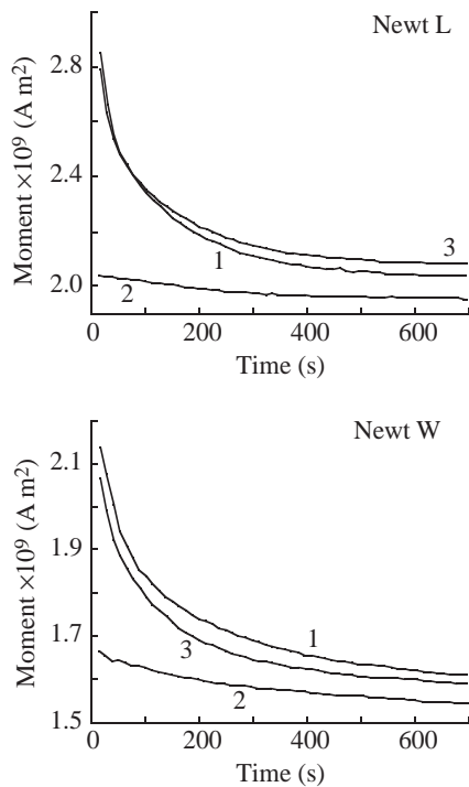
Fig. 3. Variation of the remanence acquired at low temperature monitored during zero-field heating. Néel (1949) has shown that the relaxation time for a magnetic domain will increase exponentially as the temperature is lowered. Thus, some grains that are superparamagnetic (SPM) at room temperature ( \approx 300 K) will behave as single domains (SDs) capable of retaining remanence at much lower temperature. Conversely, any net remanence held by these domains at low temperature will disappear as they warm in field-free space across their SPM/SD transition (their blocking temperature). For the first warming cycle, the sample was given an isothermal remanent magnetization (IRM) at low temperature, and the magnetization was then monitored over time (curve 1) as the sample warmed inside the field-free region of the magnetometer. Curve 2 was obtained after the sample had been cooled down, but not given an IRM. Curve 3 shows a subsequent warming cycle following the same procedure as for the first cycle. See text for more details. The progressive decrease in curves 1 and 3 compared with curve 2 suggests the presence of SPM ferromagnetic grains in the newt.
