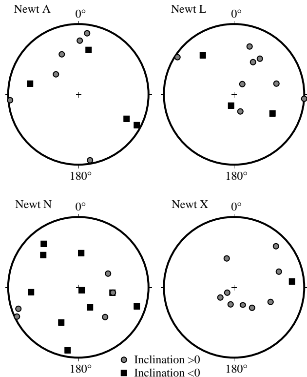
Fig. 1. Equal-area projection of mean magnetic grain directions deduced from the alternating-field (Af) demagnetization of the natural remanent magnetization (NRM). The Af demagnetization of the NRM was performed to give some idea of whether the grain magnetizations were all aligned along a preferential direction. The additive property of magnetization (a vector) is combined with the Af demagnetization to separate any non-aligned component of the magnetization. The graphic procedure used here is to view the magnetization vector directions as radiating from the center of a unit sphere, and to display the intersection of these vectors with the sphere. The sphere and the points of intersection of the vectors with it are then projected onto the horizontal plane. Filled squares are for negative inclinations (i.e. upwards relative to the horizontal plane) and grey solid circles are for positive inclinations (i.e. downwards relative to the horizontal plane). The declination is measured around the perimeter of the projection, clockwise from 0° (0° is oriented towards the nose of the newt and 180° towards the tail). The inclination is measured from 0° at the perimeter of the projection to \pm 90^\circ at the center of the projection. Each point represents the mean direction for grains with coercivity comprised between two successive steps of demagnetization. The results indicate that grain magnetizations are not aligned along a preferential direction relative to the body of the newt.
