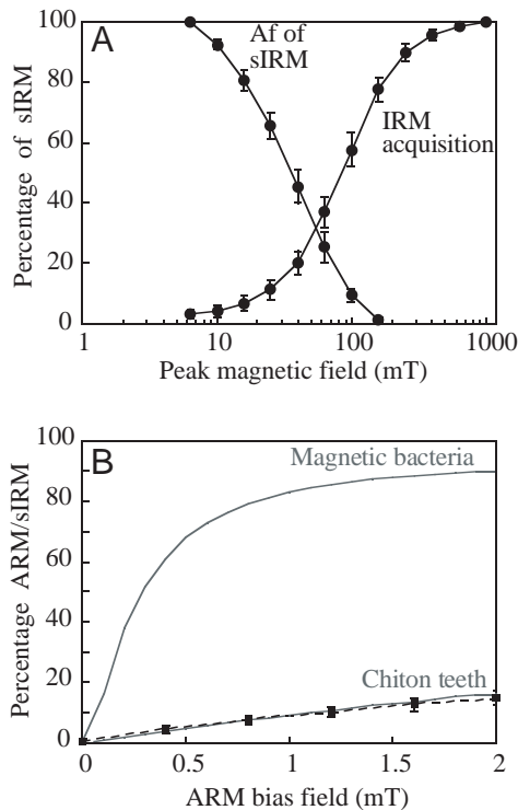
Fig. 2. Mean pattern of magnetic behavior of the newt's magnetization carriers. (A) The curve labeled 'IRM acquisition' shows the relative magnetic moment remaining after a brief exposure to a magnetic pulse of the indicated strength. The tendency of the curve to flatten at high field levels is characteristic of the magnetite–maghemite solid solution series; most other ferromagnetic minerals saturate in fields higher than 1 T. The curve labeled 'Af of sIRM' shows the progressive alternating-field demagnetization of the saturation isothermal remanent magnetization (IRM). The magnetic field value at which these two curves cross is a good estimate of the remanent coercive force (Hrc). The ordinate of the intersection point for non-interacting particles occurs at the 50% value; a depression or shift in this position is an indication of particle clumping effects. Values are means \pm s.d., N=18 . (B) The acquisition of anhysteretic remanent magnetization (ARM). The upper control curve shows data from a sample of magnetotactic bacteria in which the magnetite crystals are aligned in linear chains and have few other interparticle interactions, whereas the lower control curve is from a sample of magnetite from chiton teeth, which are single-domain crystals but are highly interacting. The filled squares joined by a dashed line represent the mean pattern ( \pm s.d., N=18 ) for the newt ferromagnetic material. This pattern suggests that the ferromagnetic grains are in small interacting clumps.
