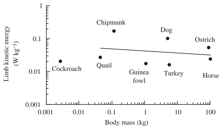
Fig. 6. Mass-specific limb kinetic energy as a function of animal mass plotted on logarithmic scales. Values are calculated using the individual species regression equations (Fedak et al. 1982) for animals theoretically moving at the same speed ( 20 \text{ cm s}^{-1} ).
