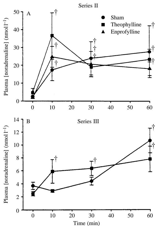
Fig. 3. Plasma [noradrenaline] of rainbow trout (A, series II) and Pacific hagfish (B, series III) in relation to exposure duration to hypoxia ( P_{W_{O_2}}=3.33 kPa in series II, P_{W_{O_2}}=1.33 kPa in series III). Animals were injected with saline (circles), theophylline (squares) or enprofylline (triangles). Time 0 values are controls. † indicates a significant difference from the control value in a given treatment ( P<0.05 ). Values are means \pm 1 S.E.M.; values of N are given in the Materials and methods section.
