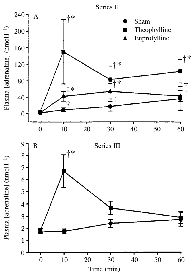
Fig. 2. Plasma [adrenaline] of rainbow trout (A, series II) and Pacific hagfish (B, series III) in relation to exposure duration to hypoxia ( P_{W_{O_2}}=3.33 kPa in series II and 1.33 kPa in series III). Animals were injected with saline (circles), theophylline (squares) or enprofylline (triangles). Time 0 values are controls. † indicates a significant difference from the control value in a given treatment. * indicates a significant difference from the value for the hypoxic sham treatment at a given sampling time ( P<0.05 ). Values are means \pm 1 S.E.M.; values of N are given in the Materials and methods section.
