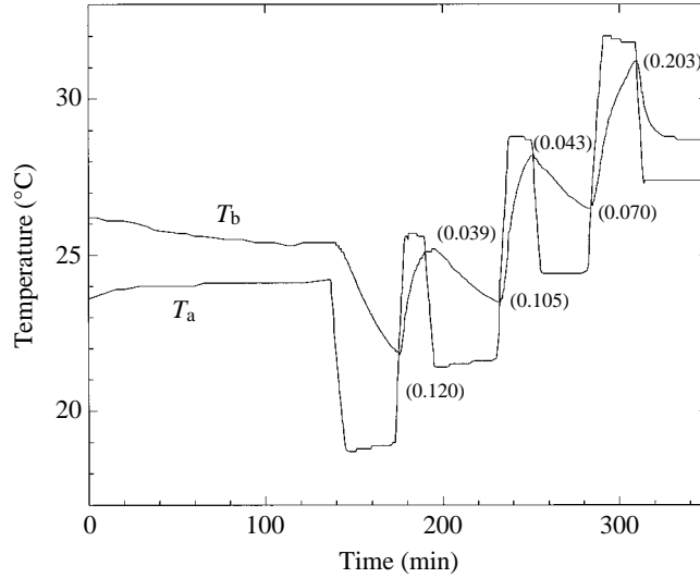
Fig. 2. Traces of T_a and T_b versus time for yellowfin no. 1 at a constant swimming speed ( 0.83 L s^{-1} ) show the typical experimental design used for all fish. The 120 min handling-recovery period and the initial drop in T_a set the stage for the subsequent cyclic changes in T_a . The k value for each T_a step change is given in parentheses.
