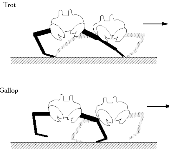
Fig. 9. Deceleration (black legs) and acceleration (stippled legs) during trotting and galloping in ghost crabs. In a trot, the flat angle of attack of the trailing leg during deceleration may make force transmission difficult. The chances of slipping would be increased or the dactylopodytes might dig deeply into the sand and hamper the animal's movement. The leading leg would have similar problems in the acceleration phase. During galloping, the trailing legs accelerate, while the leading legs largely decelerate the body (Blickhan and Full, 1987). By using the leading legs simply as passive skids, activated muscles in these legs are primarily stretched.
