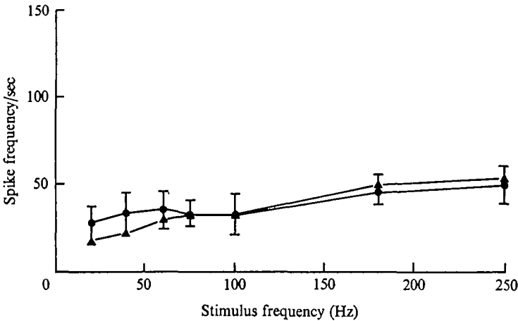
Fig. 6. As in Fig. 5 but with the stimulating electrode transferred to nerve A . Notice that the rise in the frequency of the anterior unit, which is characteristic of closure, fails to occur.
