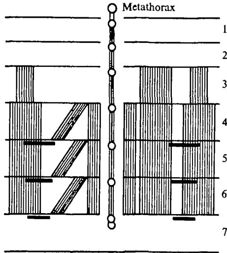
Fig. 1. A diagram of the persistent muscles and the abdominal nervous system in a diapausing pupa of Sphinx ligustri . On one side the ventral longitudinal muscles are partially removed to reveal diagonal muscles. At this stage the neuropile of the second abdominal ganglion is visible in the connective, arrested during its anterior migration to the thoracic ganglion of the adult. Abdominal segments numbered 1 to 7. Horizontal bars: gin traps.
