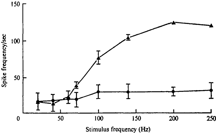
Fig. 5. The average frequency of the first ten spikes recorded in corresponding ventral motor units in segments 4 (triangles) and 5 (circles) in response to an electrical stimulus to nerve B in segment 5 at the indicated frequencies. The average frequency of the unit in the anterior segment rises with the stimulus frequency.
