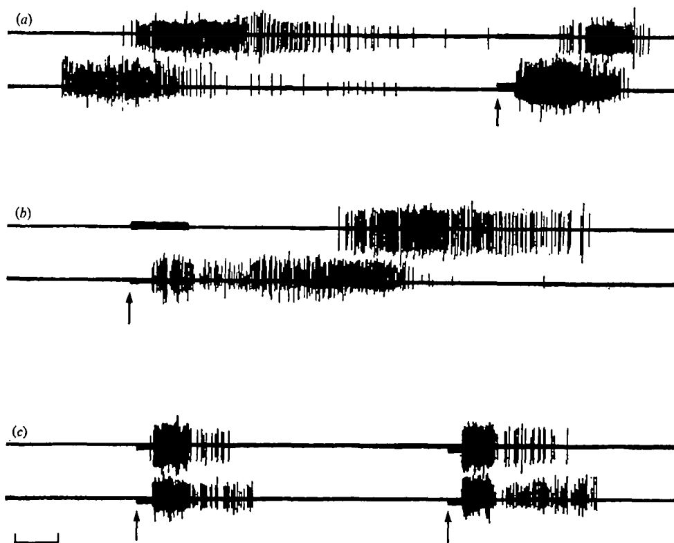
Fig. 8. The response of efferent neurones involved in closure to a high-frequency stimulus to nerve B during (a) and (b) and between (c) twirling sequences. All connexions between motor neurones and muscles were severed. Upper trace, ventral efferent neurones; lower trace, dorsal efferent neurones. Time bar: 500 msec. Stimuli (200 Hz) arrowed.
