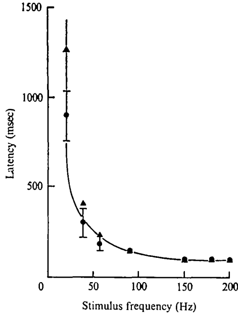
Fig. 7. The latency of the response recorded in single dorsal (circles) and ventral motor units (triangles) to stimuli to nerve B from the adjacent trap at the indicated frequencies. Each point is the average of five responses.
