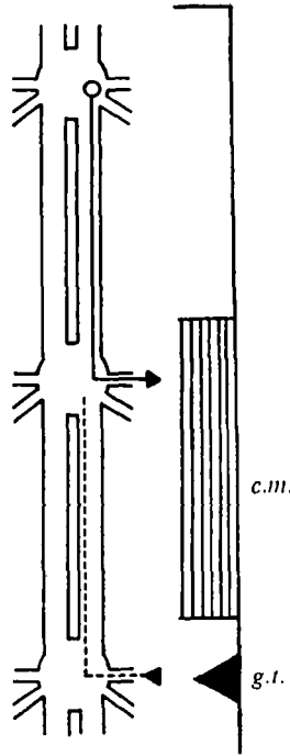
Fig. 4. The pathways of afferent (dashed line) and efferent neurones (continuous line) involved in the closure reflex, and the segments with which they are associated. Three ganglia are required for the performance of the reflex and the arrangement is repeated for each of the three pairs of gin traps. g.t. : gin trap; c.iii. : muscles which close the trap.
