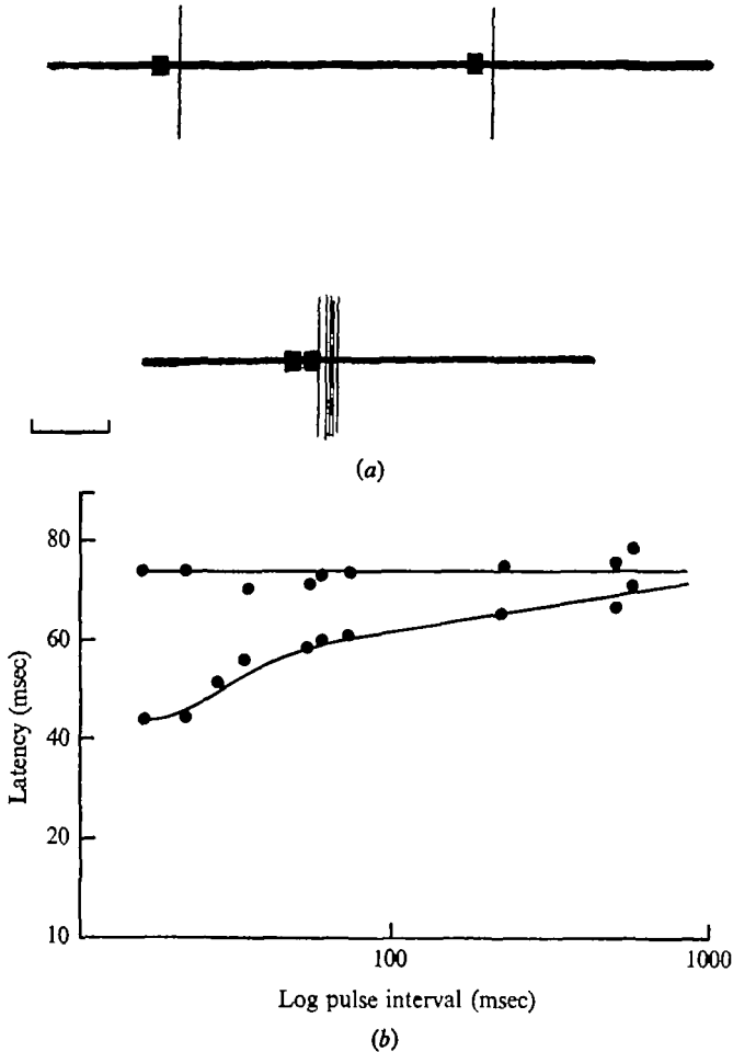
Fig. 9. (a) The latency of the response in a single ventral motor unit to two stimuli (200 Hz) to nerve B in the adjacent segment with a variable delay between the two. Time bar: 200 msec.
