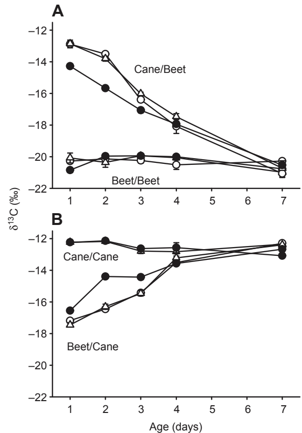
Fig. 5. Stable isotope analysis of dissected ovaries from aged female Drosophila melanogaster . Flies were reared on one of four diet regiments (larval diet/adult diet): cane/cane, cane/beet, beet/beet and beet/cane. (A) Larvae reared on cane- (upper lines) or beet-sugar medium (lower lines), and then reared on beet-sugar medium as adults. (B) Larvae reared on beet- (lower lines) or cane-sugar medium (upper lines), and then reared on cane-sugar medium as adults. Points represent mean \pm s.e.m. \delta^{13}\text{C} values of dissected ovaries; N=3 . Open circles, ovaries from UAS-diap controls; open triangles, ovaries from Lsp2-GAL4 controls; filled circles, ovaries from F1 females in which larval fat-cell death was inhibited (FCDI).
