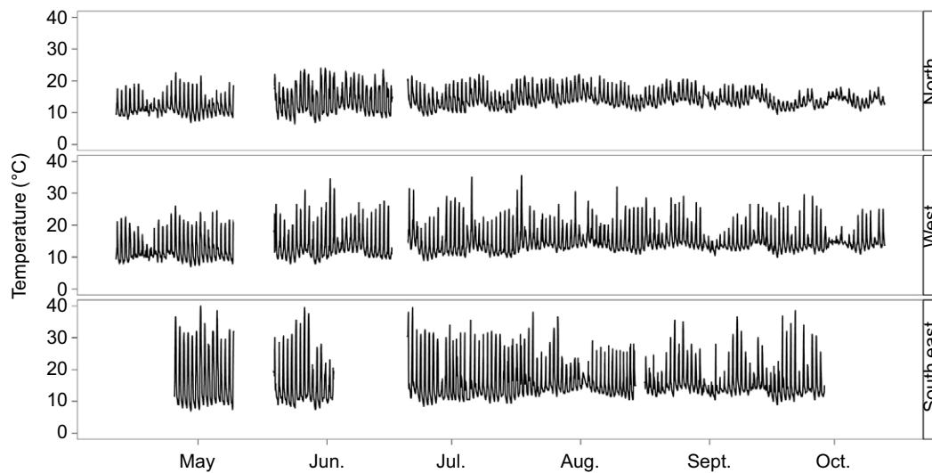
Fig. 1. Temperature profiles at Fort Ross, CA, USA, of upper intertidal rock temperatures recorded, from April to October 2011, every 10 min, at three different locations: site 1, north facing; site 2, west facing; and site 3, south-east facing. Limpets for this study were collected from all three sites.
