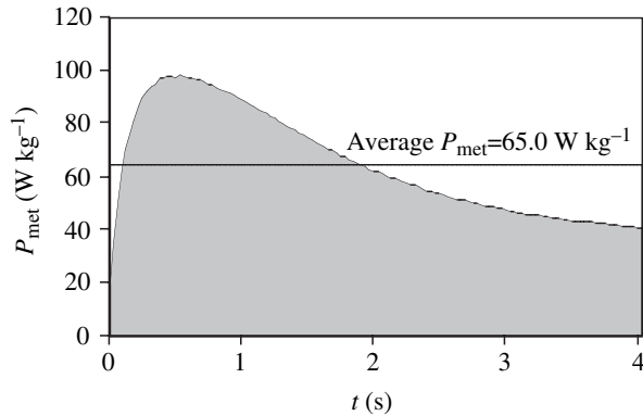
Fig. 7. Metabolic power P_{\text{met}} ( \text{W kg}^{-1} ), as calculated from the product of C_{\text{sr}} (see Fig. 6) and the speed, as a function of time t (s) for subject 7. Average power over 4 s is indicated by horizontal thin line.
