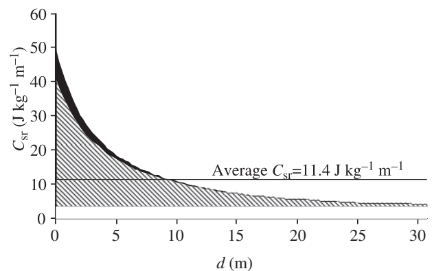
Fig. 6. Energy cost of sprint running C_{\text{sr}} ( \text{J kg}^{-1} \text{m}^{-1} ), as calculated by means of Eq. 14, as a function of the distance d (m) for subject 7. Energy cost of constant speed running is indicated by the lower horizontal thin line. Black and hatched distances between appropriate lines indicate effects of EM and ES, respectively. Upper horizontal thin line indicates average C_{\text{sr}} throughout the indicated distance.
