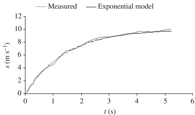
Fig. 2. Actual (gray, thick line) and modelled (black, thin line) forward speed s ( \text{m s}^{-1} ) as a function of time t (s) at the onset of a typical 100 m run for subject 7. Actual speed was accurately described by: s(t) = 10.0 * (1 - e^{-t/1.42}) . The maximal speed ( s_{\text{max}} ) was 10.0 \text{ m s}^{-1} .
