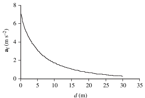
Fig. 4. The instantaneous forward acceleration a_f ( \text{m s}^{-2} ), obtained as described in the text, is plotted as a function of the distance d (m) for subject 7.
