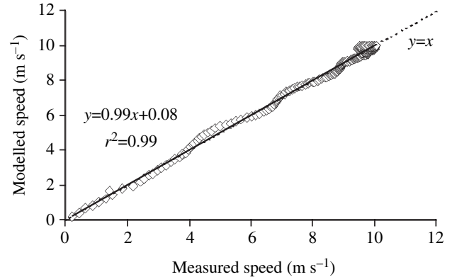
Fig. 3. Running velocity as calculated by the exponential model, as a function of the actual running speed for Subject 7. The linear relationship is reported in the figure ( N=234 ); identity line is also shown.
