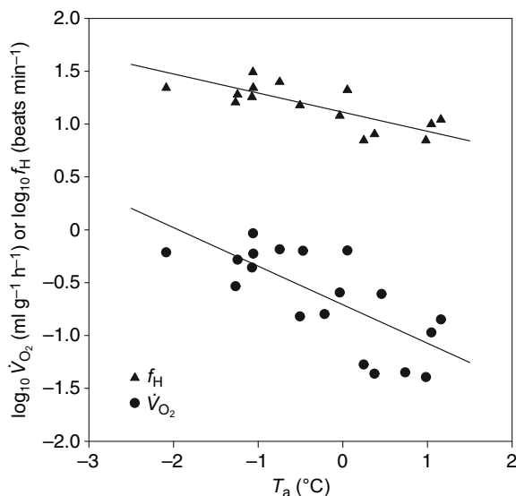
Fig. 6. f_H and \dot{V}_{\text{O}_2} as a function of T_a in thermoregulating C. gouldii during torpor. \log_{10} -transformed f_H [ \log_{10}f_H=1.11-0.18(T_a) , r^2=0.82 , P<0.001 ; n=6 , N=15 ] and \dot{V}_{\text{O}_2} [ \log_{10}\dot{V}_{\text{O}_2}=-0.71-0.37(T_a) , r^2=0.71 , P<0.001 ; n=6 , N=18 ] increased disproportionately with decreasing T_a . \dot{V}_{\text{O}_2} increased at a greater rate than f_H below 1^\circ\text{C} .
