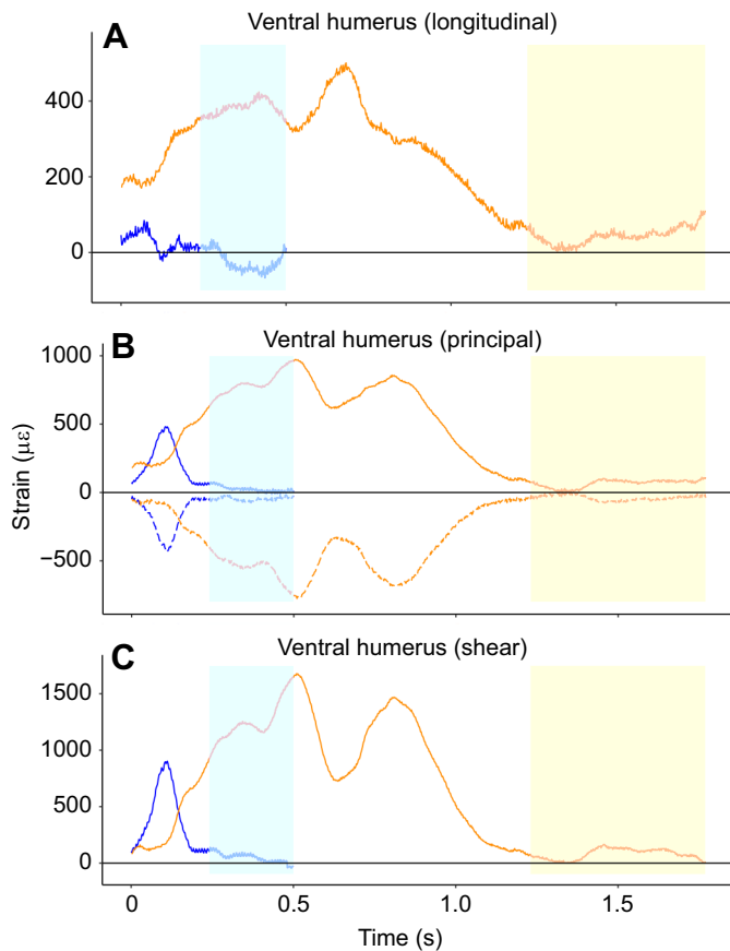
Fig. 1. Strain traces from the forelimb of a river cooter turtle ( Pseudemys concinna ). Examples of high-magnitude strain traces from turtle PC06, simultaneously recorded from a rosette gauge located on the ventral surface of the humerus during swimming and terrestrial walking. A single limb cycle from the same individual is illustrated for both behaviors. (A) Ventral longitudinal strain. (B) Ventral principal strain. (C) Ventral shear strain. Walking strains are shown in orange and swimming strains are shown in blue. Shaded regions indicate the recovery (protraction) phase of the limb cycle for each locomotor behavior (walking in yellow, swimming in light blue). Compressive principal strain is represented by a dashed line. Note the duration of the swimming cycle is approximately half that of the walking cycle. \mu\epsilon , microstrain.
