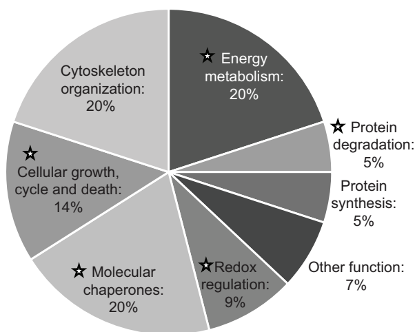
Fig. 4. Gene ontology classification of proteins generally detected in comparative proteomics. Each of the 44 generally detected proteins is assigned to only one functional category. The percentage of these proteins in each functional category is shown. Adapted from Wang et al. (2009b). Stars indicate that this functional category is also part of the minimal stress proteome defined by Kültz (2005).
