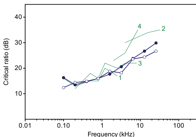
Fig. 3. Underwater and in-air critical ratios for two spotted seals measured in the presence of octave-band masking noise. Underwater critical ratios are shown for Amak (filled circles) and in-air critical ratios are shown for Tunu (open circles) at nine frequencies. Also plotted are underwater critical ratios for harbor [1, N=1 (Southall et al., 2000)] and ringed seals [2, N=2 (Terhune and Ronald, 1975b)], and aerial critical ratios for harbor [3, N=1 (Southall et al., 2003)] and harp seals [4, N=1 (Terhune and Ronald, 1971)].
