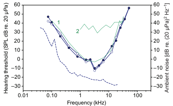
Fig. 2. Aerial audiograms for two spotted seals, Amak (filled circles) and Tunu (open circles), obtained using psychophysical methods. Ambient noise in the acoustic testing chamber is plotted as a dashed line corresponding to the right-hand y-axis. The noise profile comprises power spectral density levels [in dB re. (20 μPa) 2 Hz -1 ] calculated from the median of 1/3-octave band 50th percentile levels measured across all sessions. Previously published thresholds are shown for harbor seals [1, N=1 (Reichmuth et al., 2013)] and harp seals [2, N=1 (Terhune and Ronald, 1971)]. SPL, sound pressure level.
