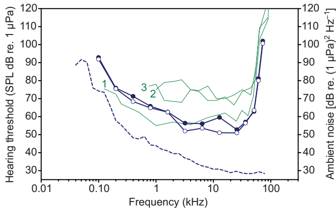
Fig. 1. Underwater audiograms for two spotted seals, Amak (filled circles) and Tunu (open circles), obtained using psychophysical methods. Ambient noise in the underwater testing enclosure is plotted as a dashed line corresponding to the right-hand y-axis. The ambient noise profile comprises power spectral density levels [in dB re. (1 μPa) 2 Hz -1 ] calculated from the median of 1/3-octave band 50th percentile levels measured across all sessions. For comparison, behavioral audiograms are also shown for harbor seals [1, N=2 (Kastelein et al., 2009)], ringed seals [2, N=2 (Terhune and Ronald, 1975a)] and harp seals [3, N=1 (Terhune and Ronald, 1972)]. SPL, sound pressure level.
